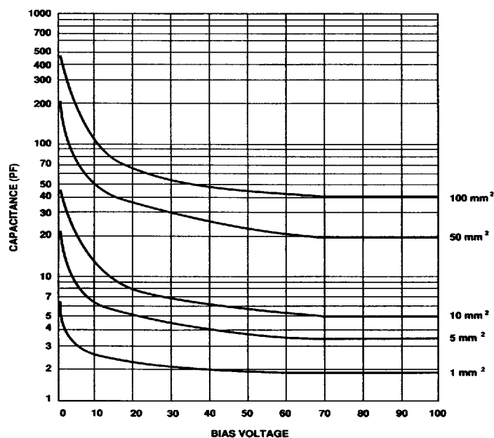
Fig.20 SERIES 3T - TYPICAL CAPACITANCE VERSUS BIAS VOLTAGE FOR A GIVEN DETECTOR AREA
