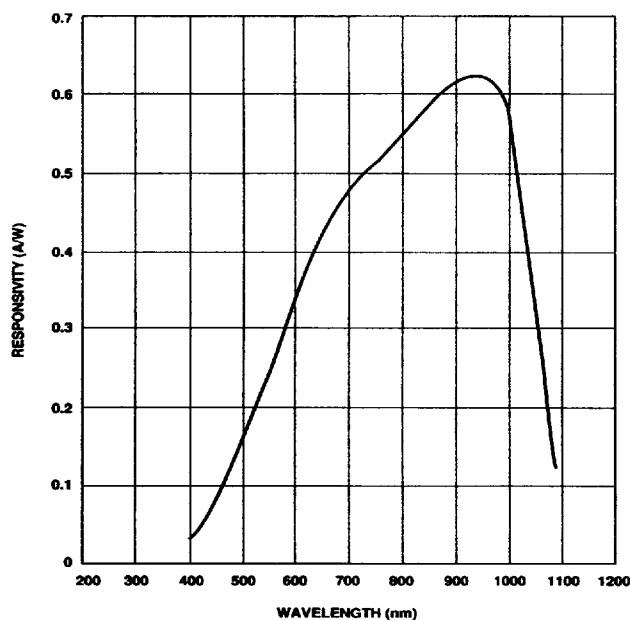
Fig.19 SERIES 3T - TYPICAL SPECTRAL RESPONSE
