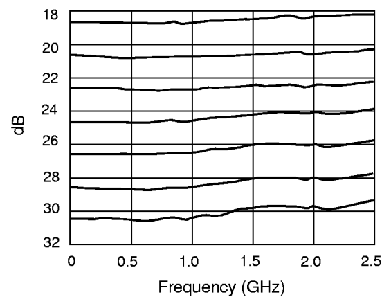
Attenuation 18 dB to 30 dB
