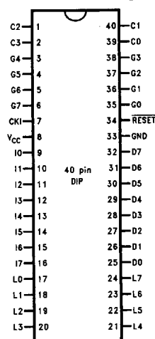
Dual-In-Line Package
