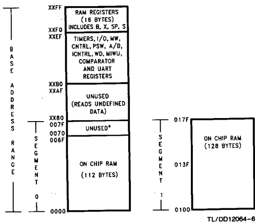
FIGURE 4. RAM Organization
