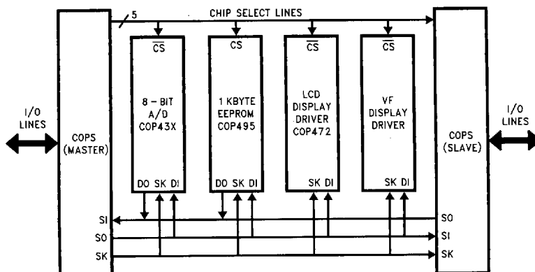
FIGURE 17. MICROWIRE/PLUS Application
