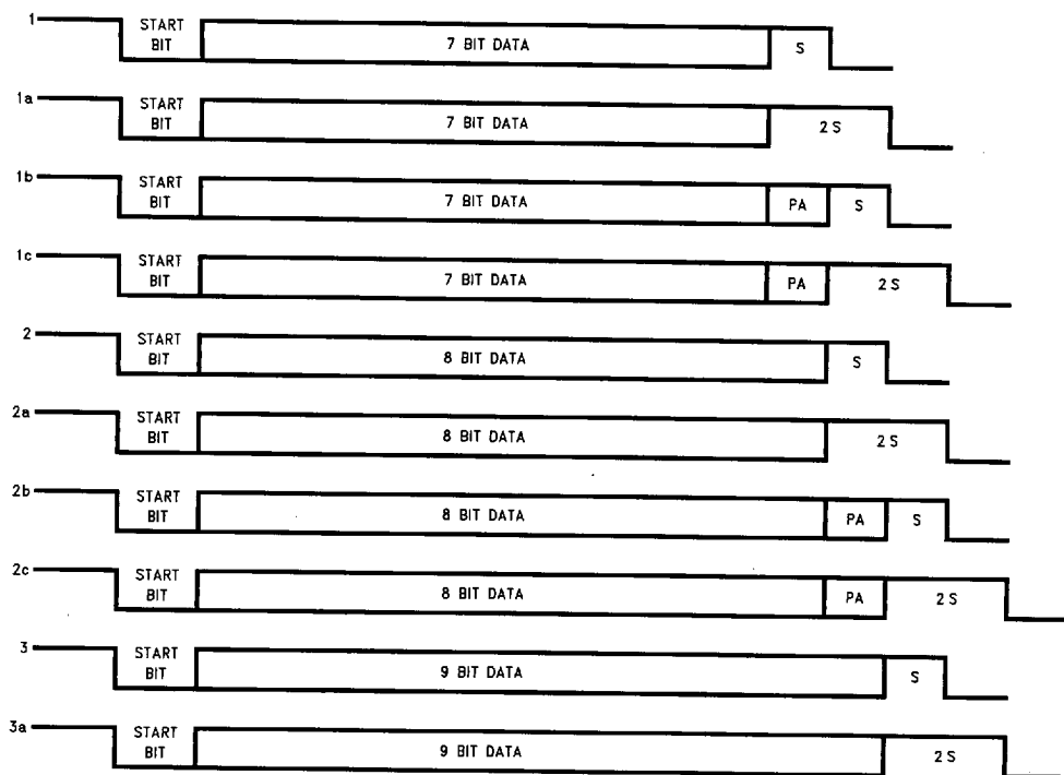
FIGURE 12. Framing Formats
