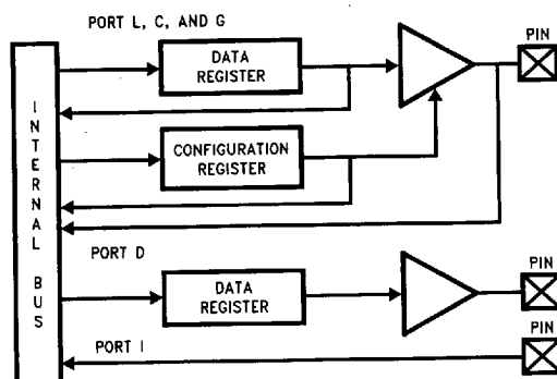
FIGURE 3. I/O Port Configurations
