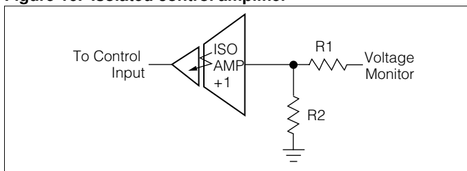
Figure 16. Isolated control amplifier
