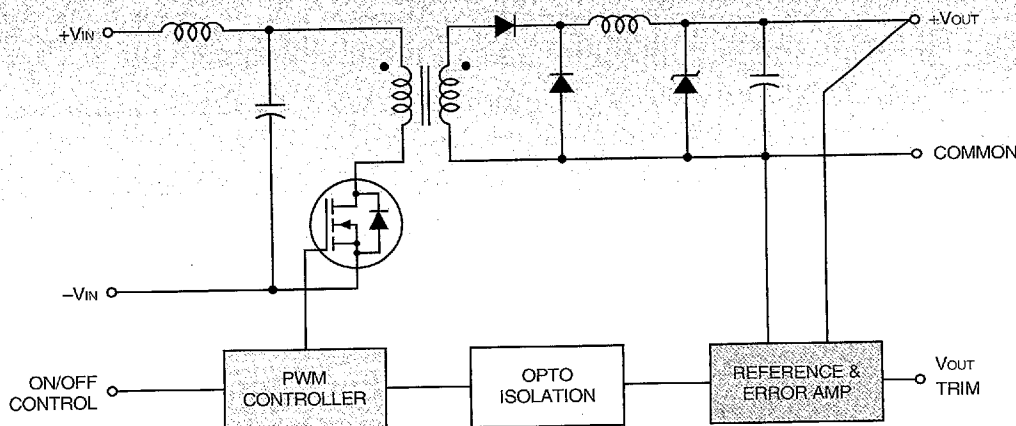
Figure 1. Simplified Schematic
