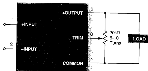
Figure 2a. Trim Connections Using a Trimpot
