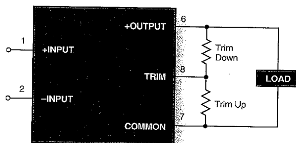
Figure 2b. Trim Connections Using Fixed Resistors
