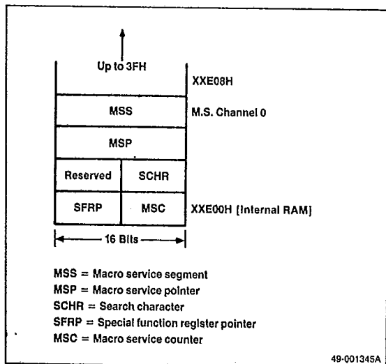
Figure 12. Macroservice Channels
