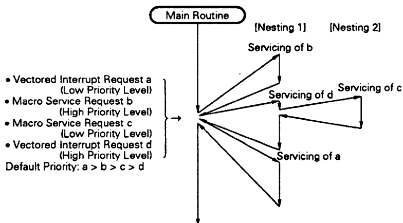
Fig. 3-2 Servicing Example for Simultaneous Occurred Interrupt Request
