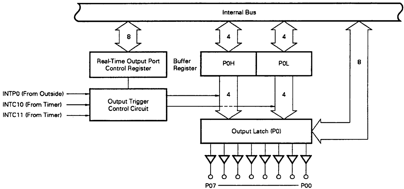
Fig. 2-4 Real-Time Output Port Block Diagram
