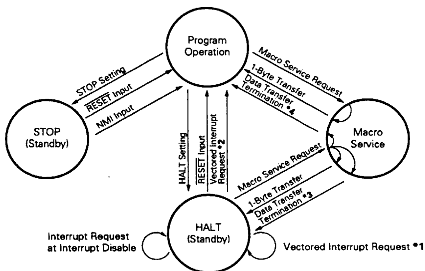
Fig. 3-5 Standby Status Flow
