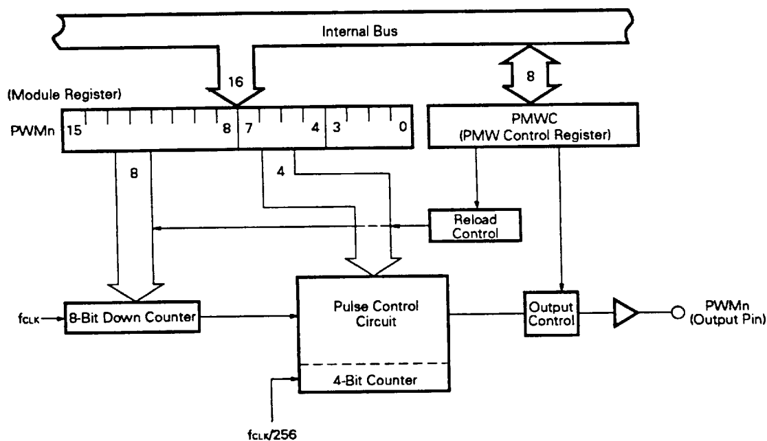
Fig. 2-6 PWM Output Unit Block Diagram (n = 0, 1)
