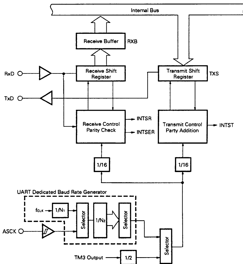
Fig. 2-10 Asynchronous Serial Interface Block Diagram
