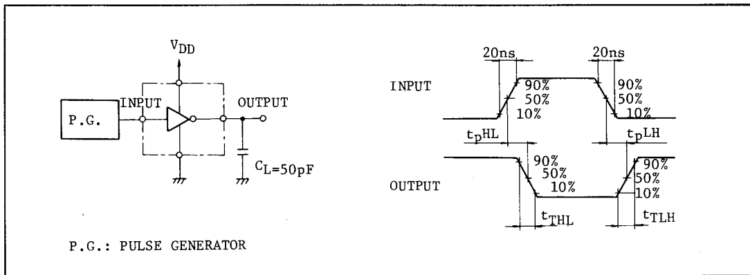
SWITCHING TIME TEST CIRCUIT AND WAVEFORM
