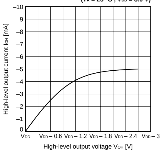
I OH vs V OH Characteristic Example ( \overline{\text{LED}} ) (T A = 25 °C, V DD = 3.0 V)
