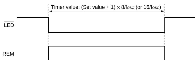
Figure 4-2. Timer Output (When Carrier is Not Output)
