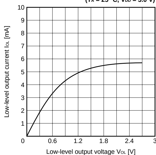
I OL vs V OL Characteristic Example (REM, \overline{\text{LED}} ) (T A = 25 °C, V DD = 3.0 V)
