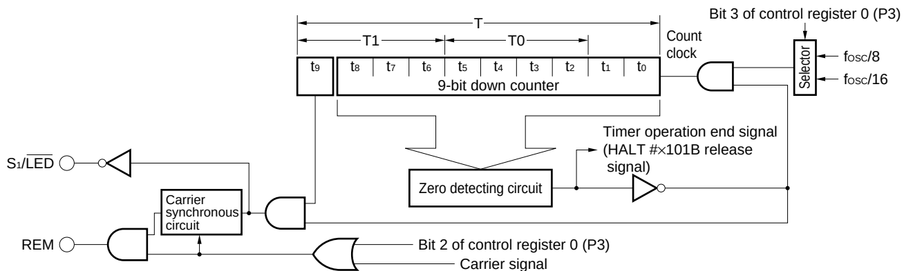
Figure 4-1. Timer Configuration
