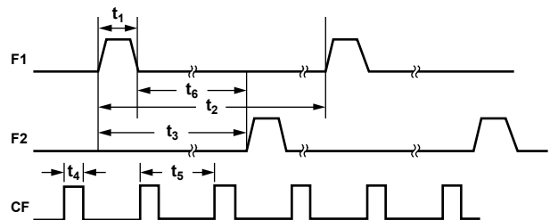
Figure 2. Timing Diagram for Frequency Outputs
