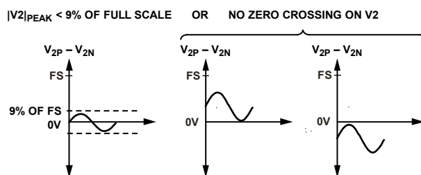
Figure 33. Missing Neutral Detection
