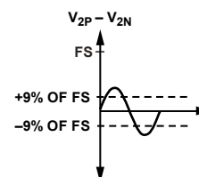
Figure 34. Return to Normal Mode after Missing Neutral Detection
