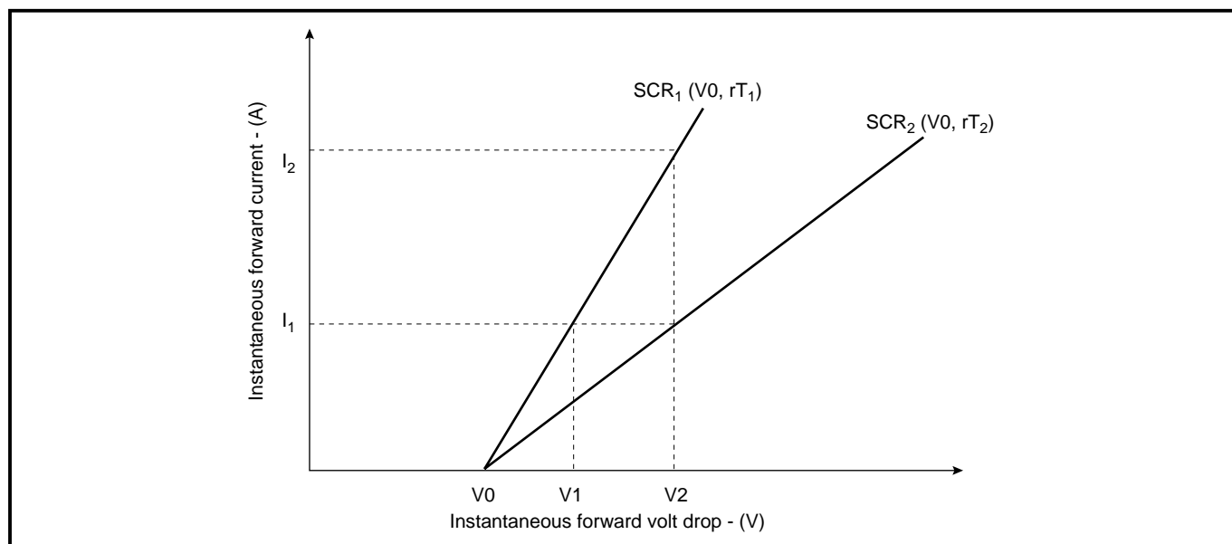
Fig. 1 Total current is divided between the two SCRs
