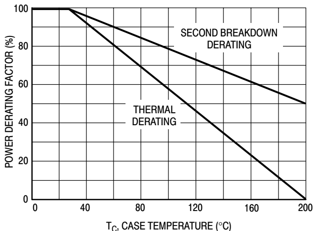
Figure 15. Power Derating
