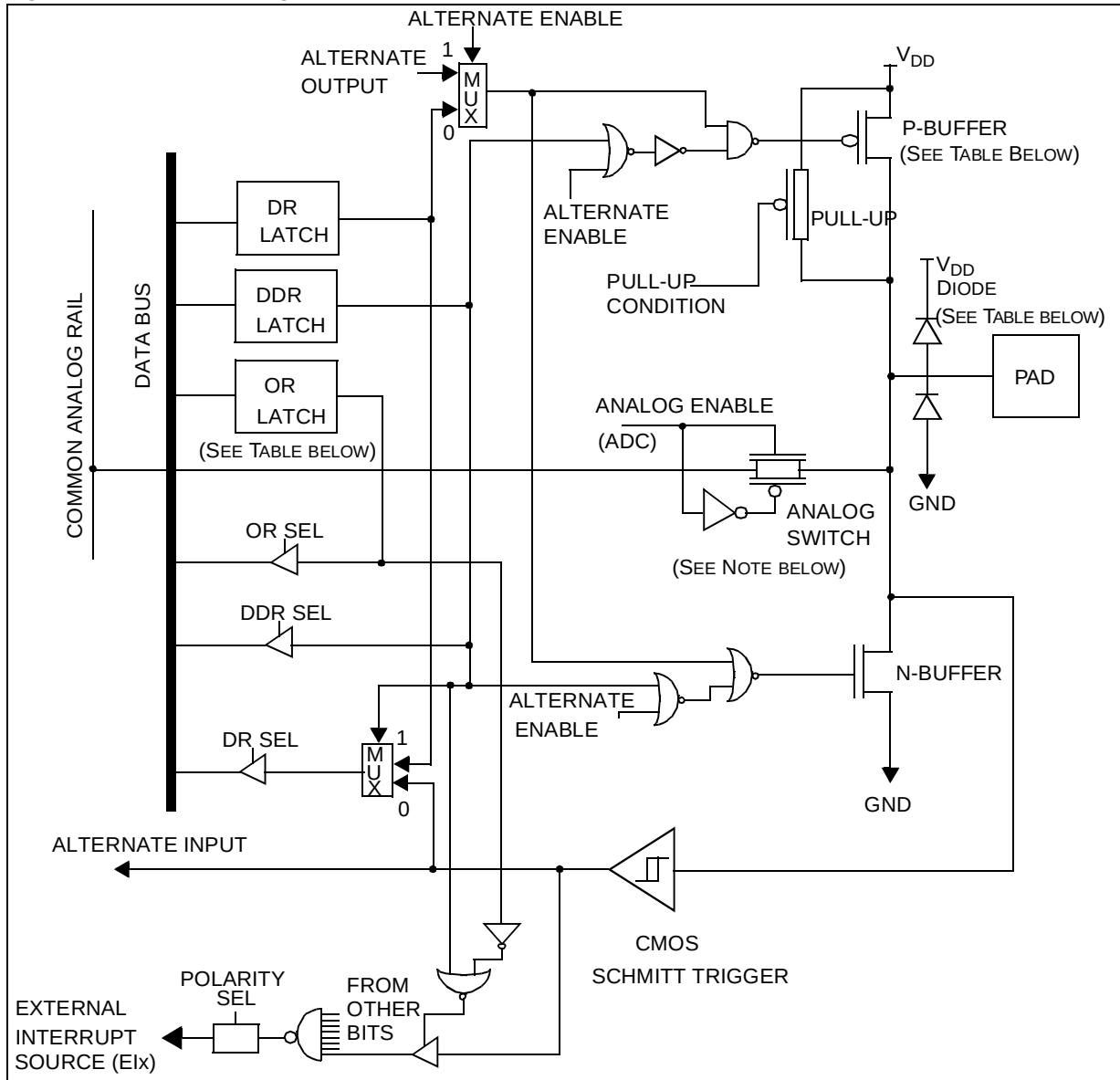
Figure 20. I/O Block Diagram
