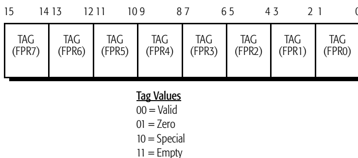
Figure 14. FPU Tag Word Register
