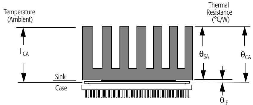
Figure 110. Thermal Model
