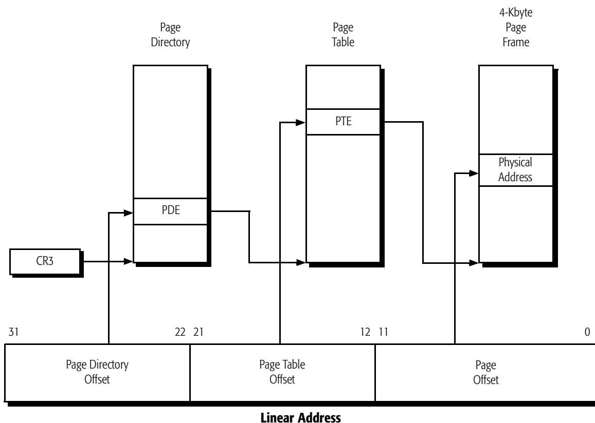
Figure 45. 4-Kbyte Paging Mechanism
