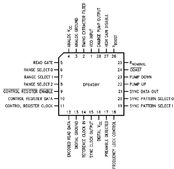
FIGURE 1. DP8459 in 28-Pin Plastic Chip Carrier (PCC) V-Type Package Order Number DP8459V-10 or DP8459V-25
