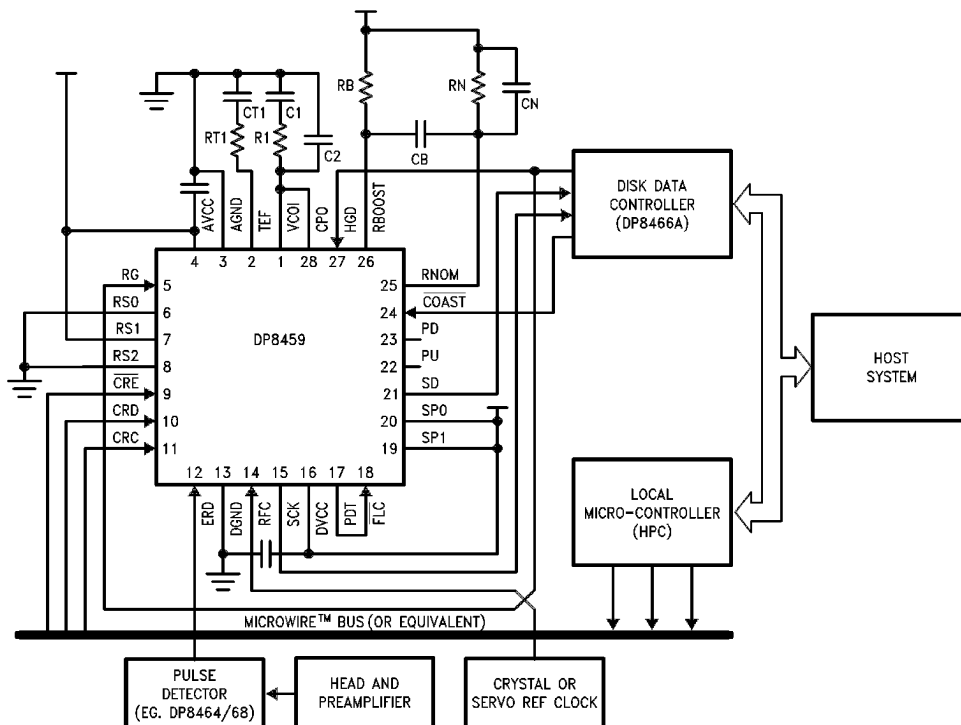
FIGURE 17. DP8459 in a Typical System Configuration
