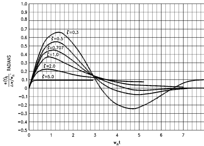
FIGURE 18. Transient Phase-Error Versus the Dimensionless Parameter \omega_n t Due to a Step in Frequency for Various Loop Damping Factors, \zeta (from Ref. 4 by Permission of L. A. Hoffman)
