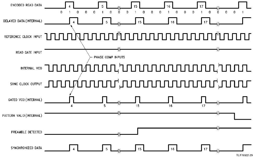
FIGURE 28. Occurrence of Preamble Detection; 4T Pattern, Frequency Lock not Employed (Soft Sectoring)
