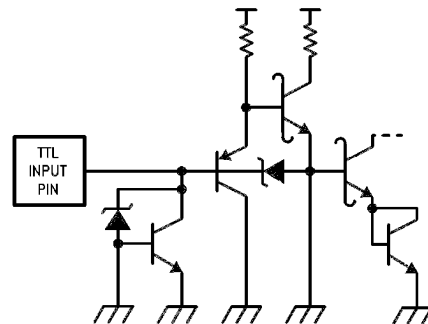
FIGURE 34. Typical TTL Digital Input
