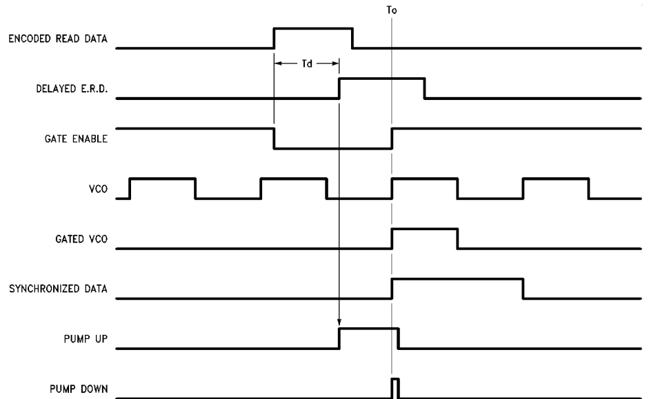
FIGURE 8. Capture of Early-Shifted ENCODED READ DATA Pulse
