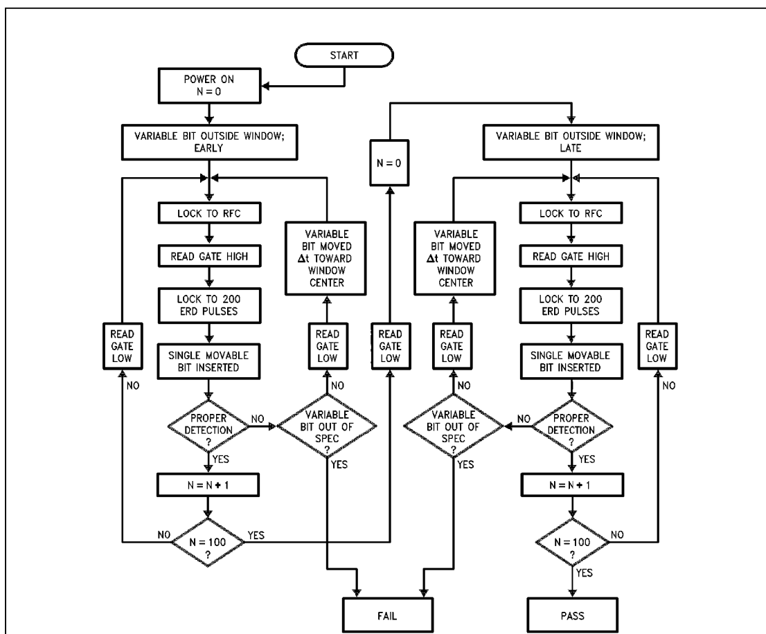
FIGURE 24. DP8459 Static Window Truncation Test Flow Chart
