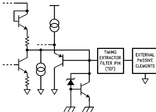
FIGURE 36. Timing Extractor Filter Pin Circuit Configurations
