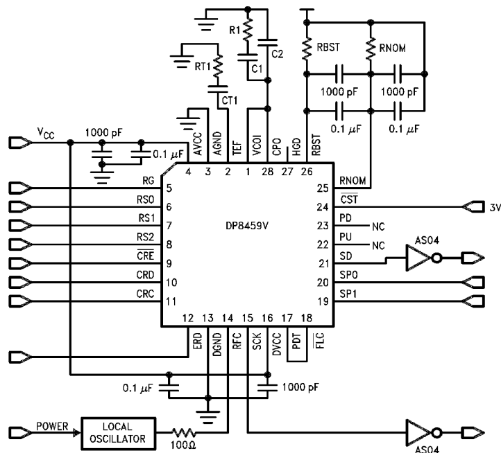
FIGURE 23. DP8459 Window Measurement Configuration
