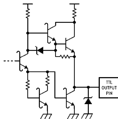
FIGURE 31. Typical TTL Digital Output
