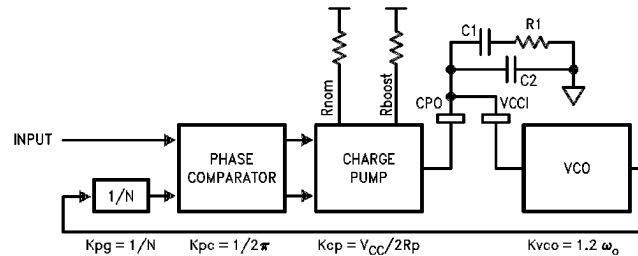
FIGURE 16. Basic DP8459 Phase Locked Loop Block Diagram
