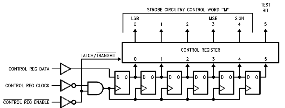
FIGURE 13. Control Register
