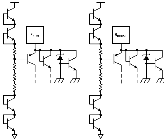
FIGURE 33. R_{NOMINAL} and R_{BOOST} Pin Configurations
