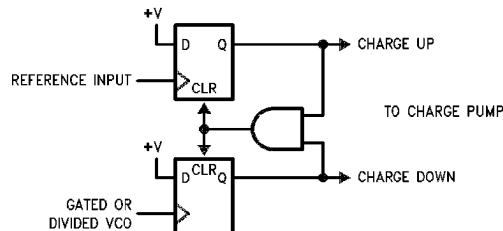
FIGURE 11. Simplified Digital Phase-Frequency Comparator
