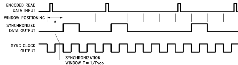
FIGURE 21. Synchronization Window
