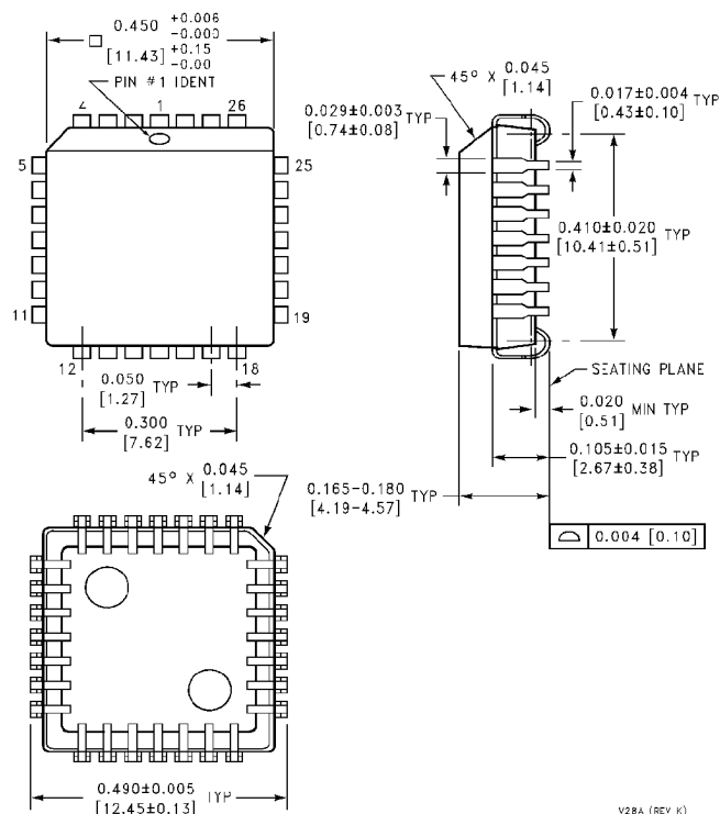
Plastic Chip Carrier Package (V) Order Number DP8459V-10 or DP8459V-25NS Package Number V28A
