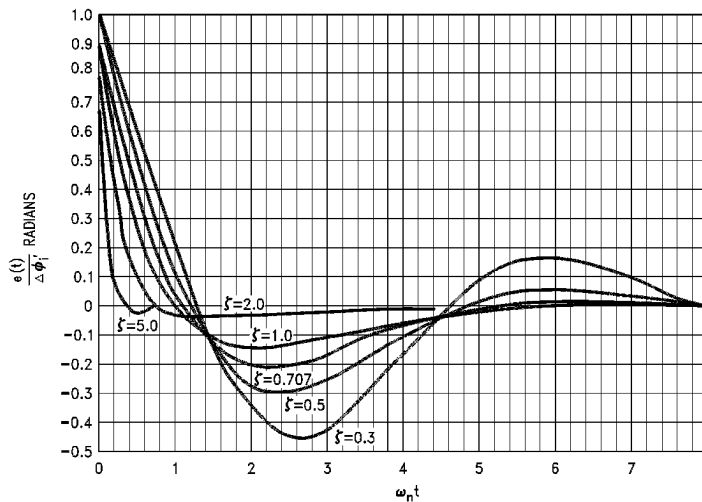
FIGURE 19. Phase-Error Versus the Dimensionless Parameter \omega_n t Due to a Step in Phase for Various Loop Damping Factors, \zeta (from Ref. 4 by Permission of L. A. Hoffman)
