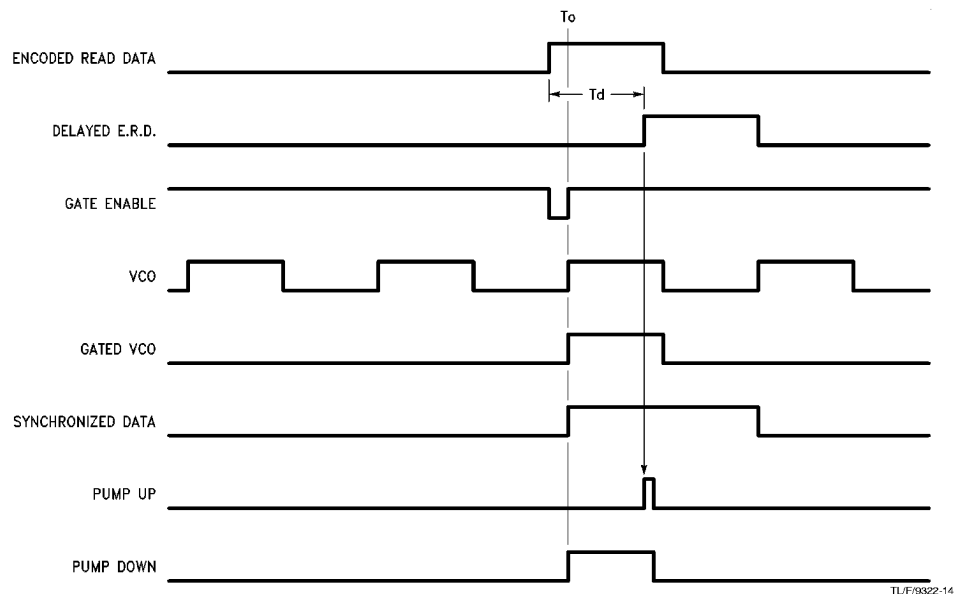
FIGURE 9. Capture of Late-Shifted ENCODED READ DATA Pulse
