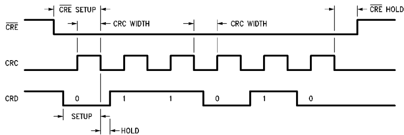
FIGURE 14. Microwire Compatible Control Register Serial Load Timing Diagram
