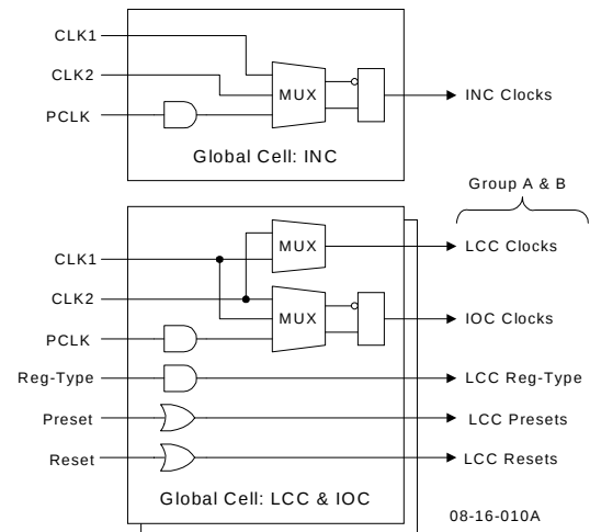
Figure 10. Global Cells
