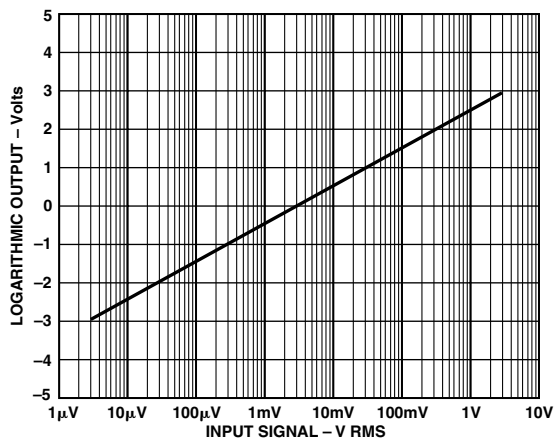
Figure 30. V_{\text{LOG}} Is Essentially Linear Over the Full 120 dB Range
