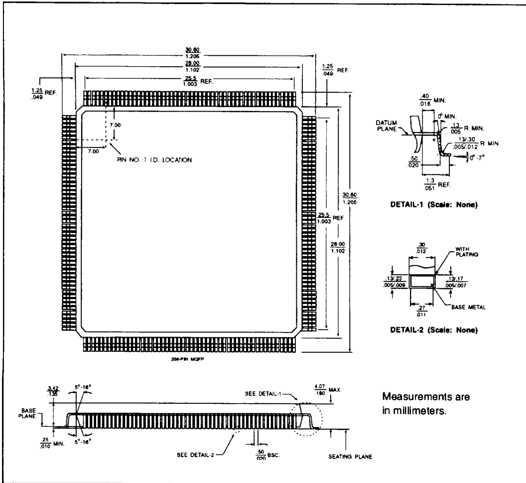
FIGURE 8-2 208-PIN MQFP
