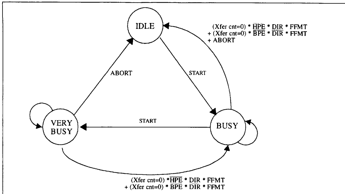
FIGURE 5-19 HOST PIPELINE CONTROL
