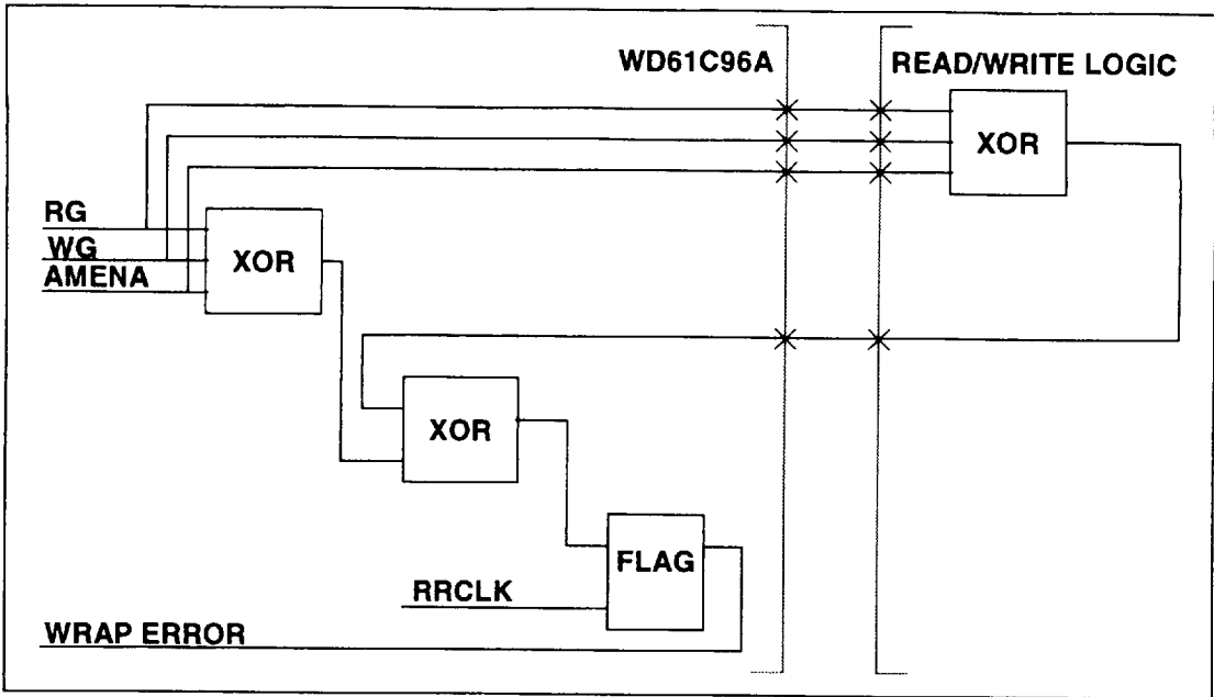
FIGURE 5-26 WRAP PATH
