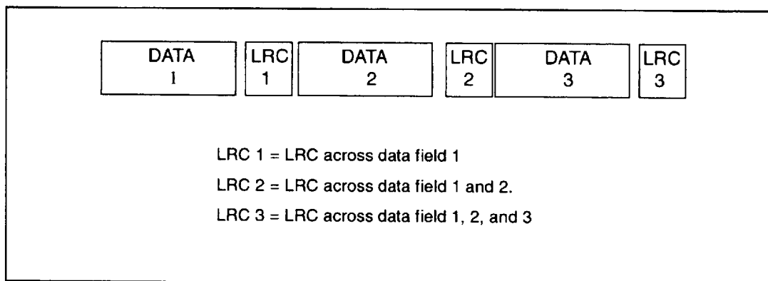
FIGURE 5-25 LRC EXAMPLE
