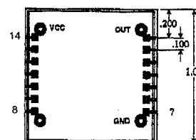
Z2 J-leads
