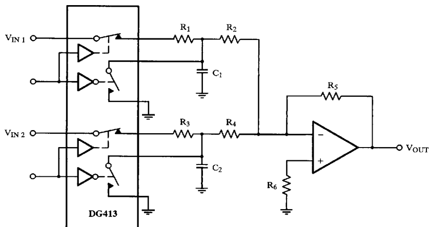
Figure 8. Summing Amplifier
