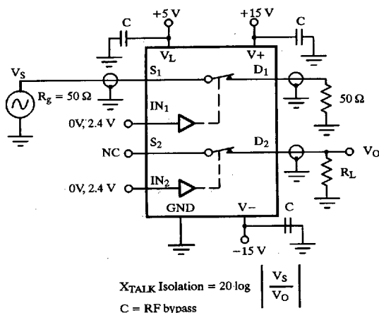
Figure 5. Crosstalk
