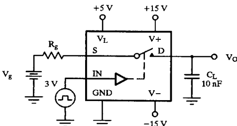
Figure 4. Charge Injection
