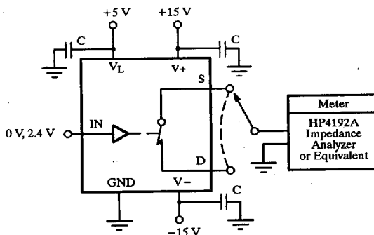
Figure 7. Source/Drain Capacitances
