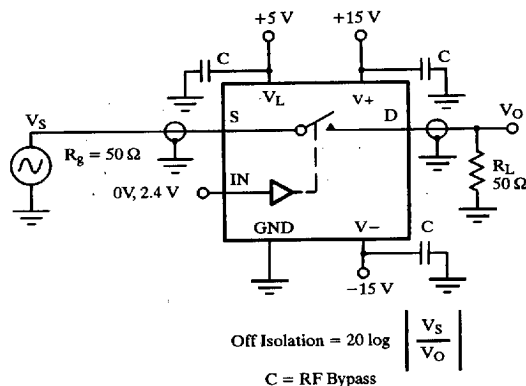
Figure 6. Off Isolation
