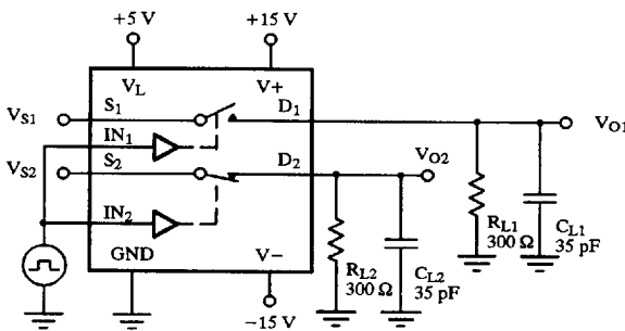
Figure 3. Break-Before-Make (DG413)
