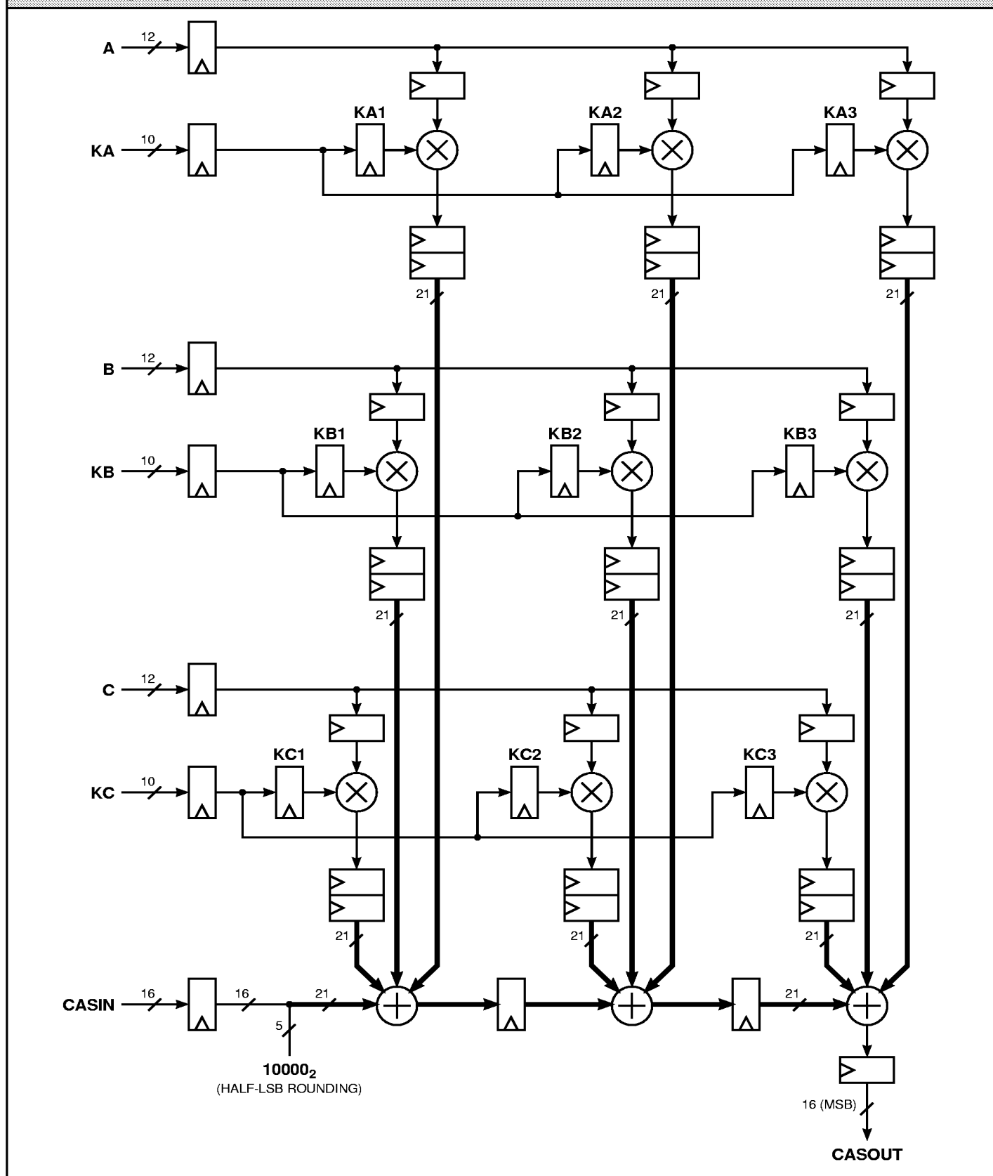
FIGURE 4. 3 x 3-PIXEL CONVOLVER — MODE 10
