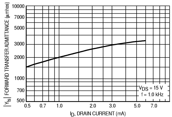
Figure 5. V_{GS(off)} = 4.0 Volts
