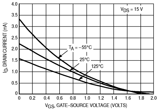
Figure 1. V_{GS(off)} = 2.0 Volts
