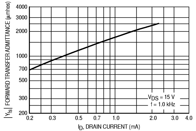
Figure 4. V_{GS(off)} = 2.0 Volts
