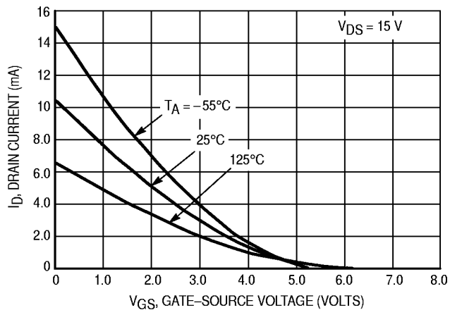
Figure 3. V_{GS(off)} = 5.0 Volts
