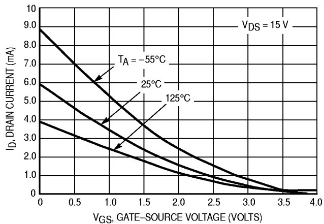
Figure 2. V_{GS(off)} = 4.0 Volts
