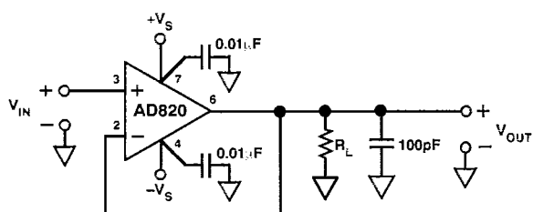
Figure 24. Unity-Gain Follower
