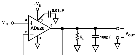
Figure 30. Unity-Gain Follower
