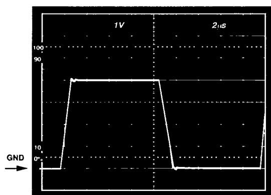
Figure 26. V_S = +5\text{ V} , 0 V; Unity Gain Follower Response to 0 V to 4 V Step
