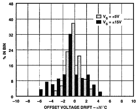
Figure 2. Typical Distribution of Offset Voltage Drift (120 Units)
