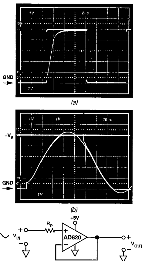
Figure 36. (a) Response with R_P = 0 ; V_{IN} from 0 to +V_S (b) V_{IN} = 0 to +V_S + 200 mV V_{OUT} = 0 to +V_S R_P = 49.9 k \Omega
