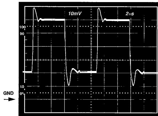
Figure 33. V_S = +5\text{ V}, 0\text{ V} ; Unity Gain Follower Response to 40 mV Step Centered 40 mV Above Ground
