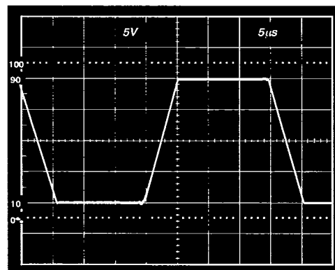
Figure 27. Large Signal Response Unity Gain Follower; V_S = \pm 15\text{ V} , R_L = 10\text{ k}\Omega
