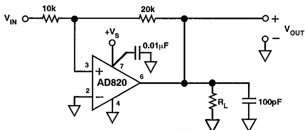
Figure 31. Gain of Two Inverter
