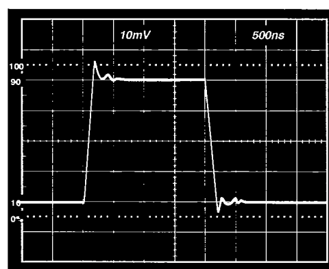
Figure 28. Small Signal Response Unity Gain Follower; V_S = \pm 15\text{ V} , R_L = 10\text{ k}\Omega
