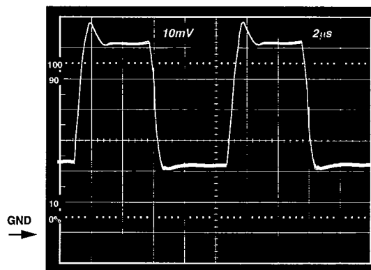
Figure 34. V_S = +5\text{ V}, 0\text{ V} ; Gain of Two Inverter Response to 20 mV Step, Centered 20 mV Below Ground
