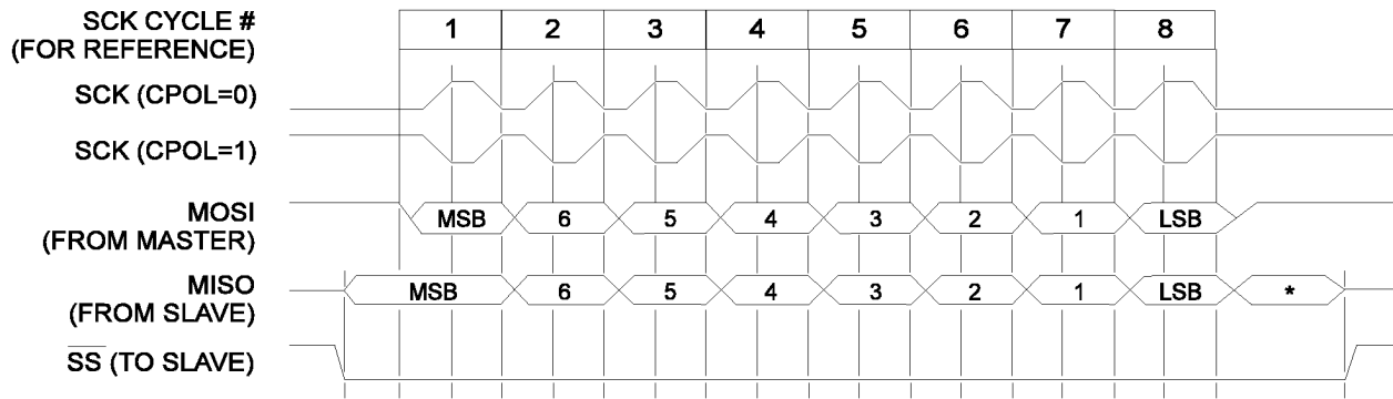
Figure 41. SPI Transfer Format with CPHA = 0
