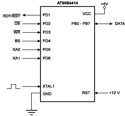
Figure 62. Parallel Programming
