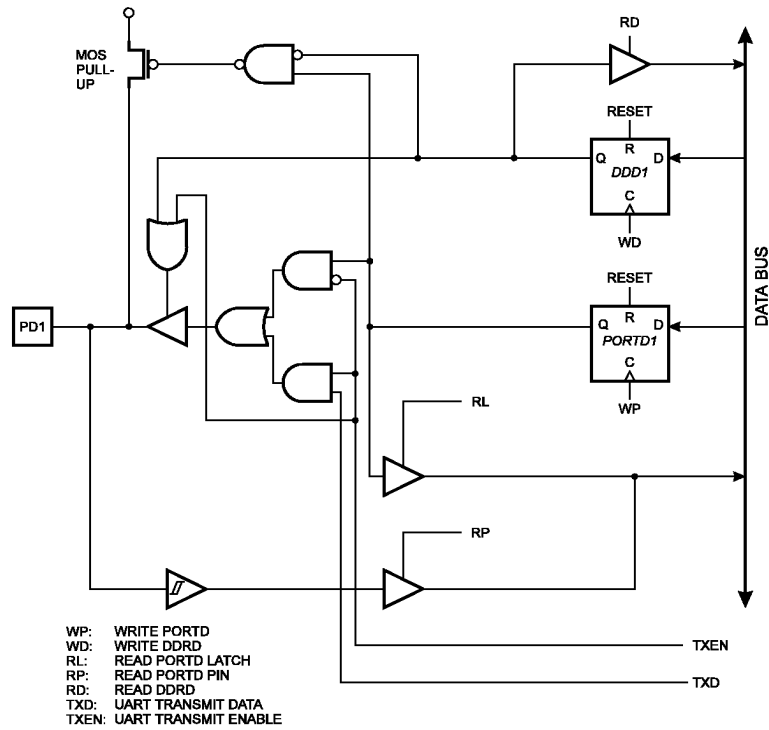
Figure 56. PORTD Schematic Diagram (Pin PD1)
