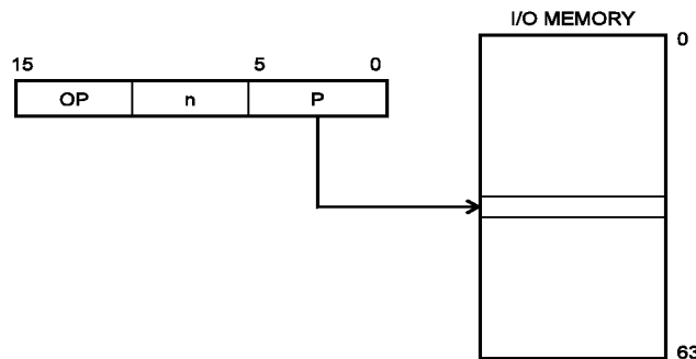
Figure 11. I/O Direct Addressing
