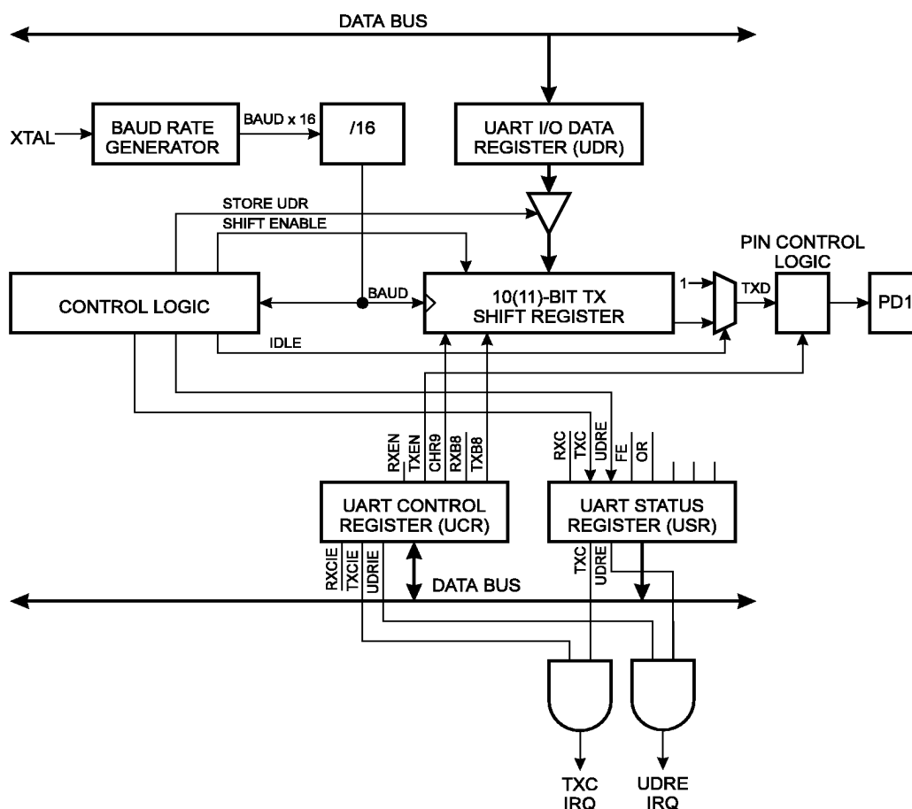
Figure 43. UART Transmitter
