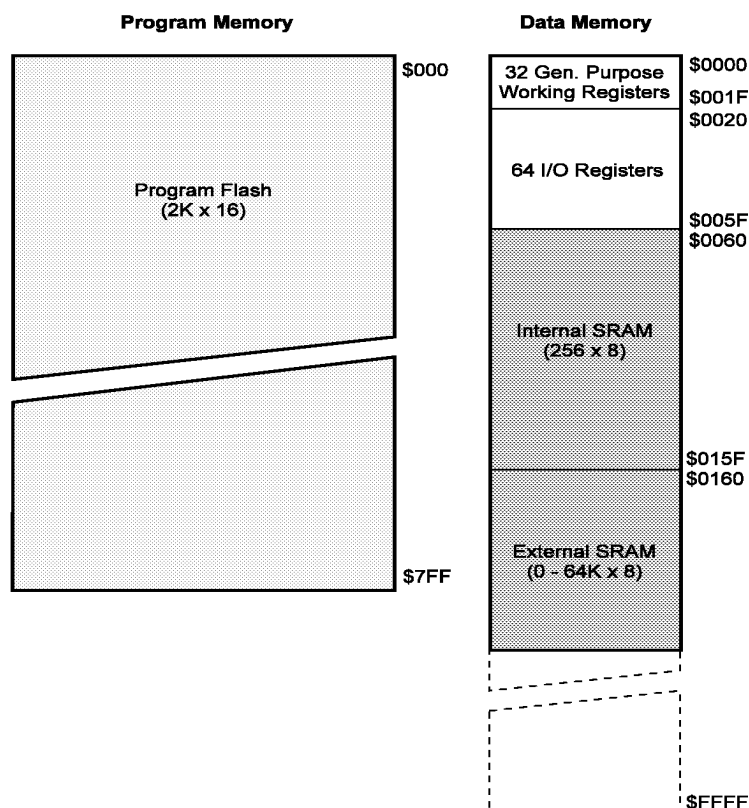
Figure 5. Memory Maps
