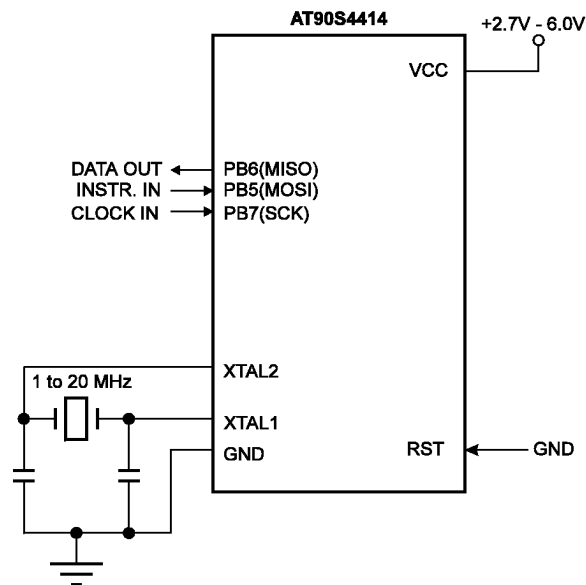
Figure 66. Serial Programming and Verify
