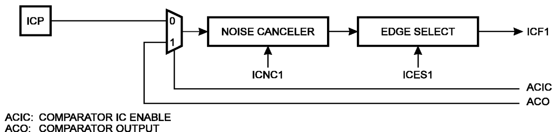
Figure 35. ICP Pin Schematic Diagram
