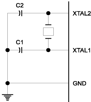
Figure 2. Oscillator Connections
