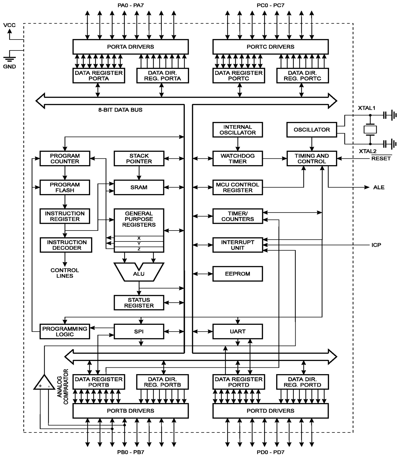
Figure 1. The AT90S4414 Block Diagram
