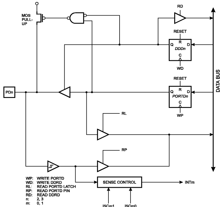
Figure 57. PORTD Schematic Diagram (Pins PD2 and PD3)
