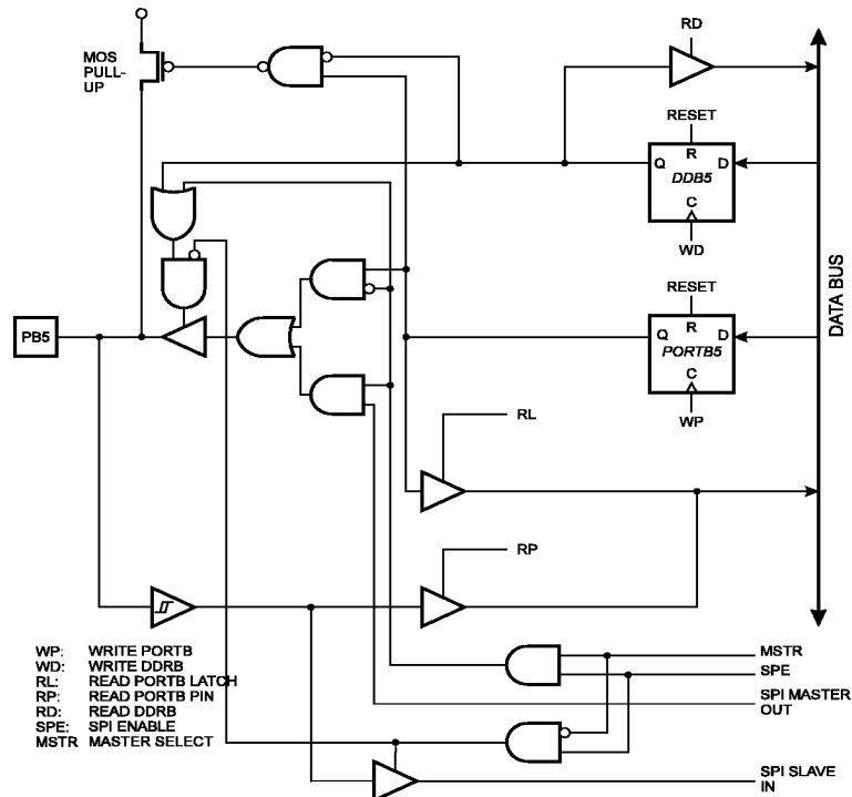
Figure 51. PORTB Schematic Diagram (Pin PB5)
