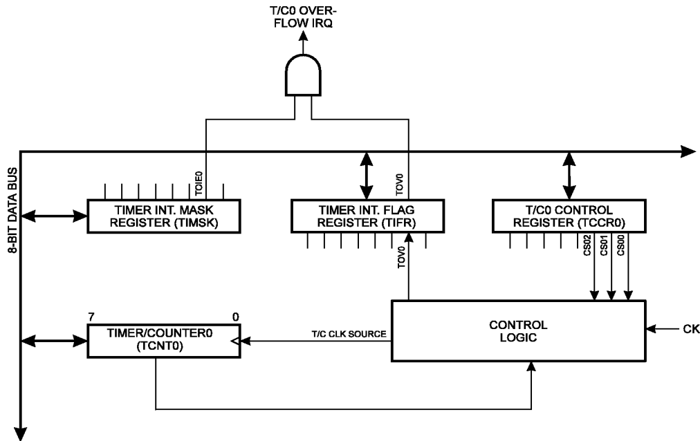
Figure 33. Timer/Counter0 Block Diagram
