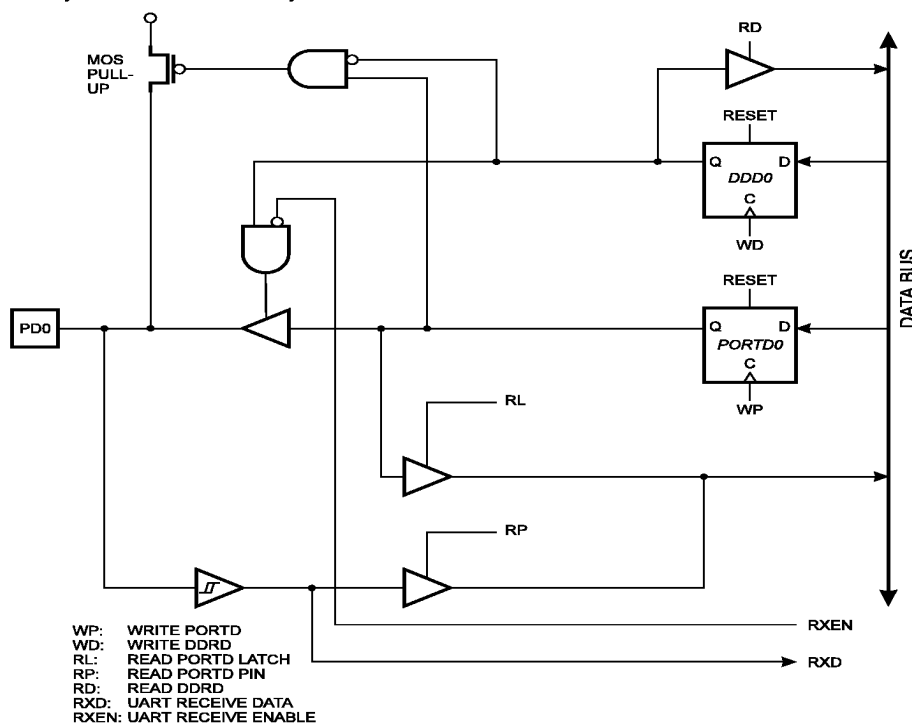
Figure 55. PORTD Schematic Diagram (Pin PD0)
