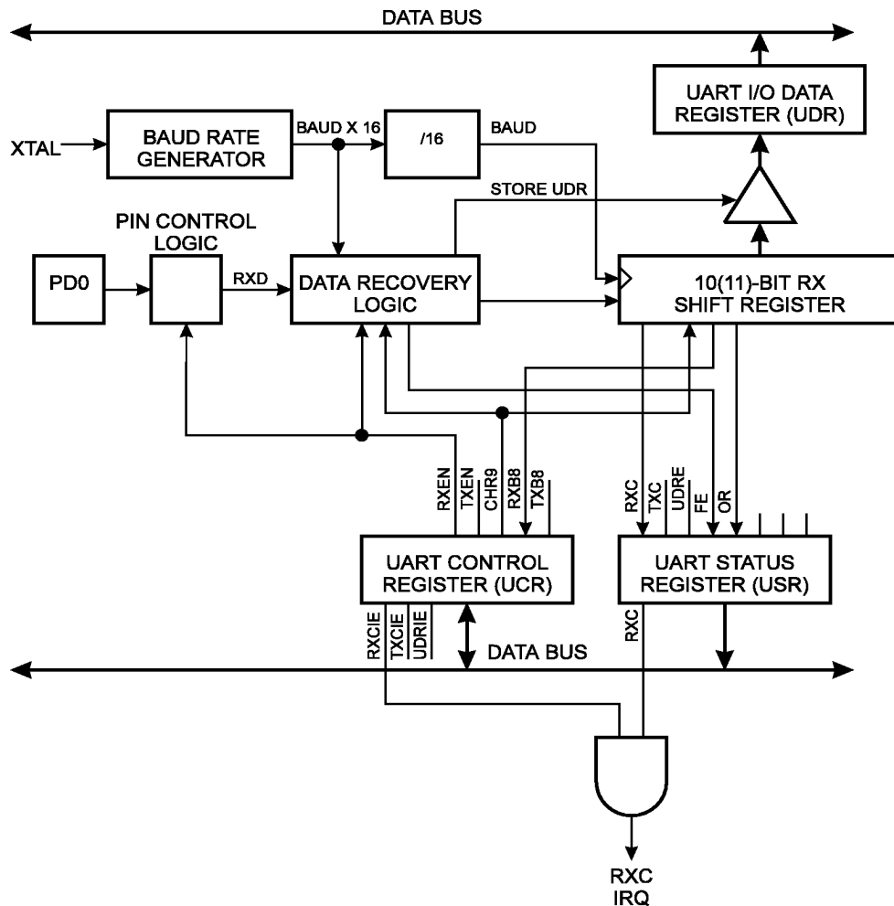
Figure 44. UART Receiver
