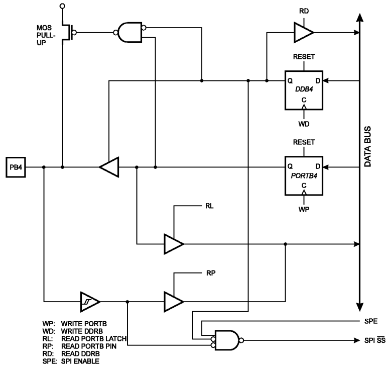
Figure 50. PORTB Schematic Diagram (Pin PB4)
