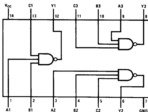
Dual-In-Line Package
