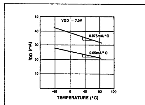
Fig.16 Power supply current vs temperature
