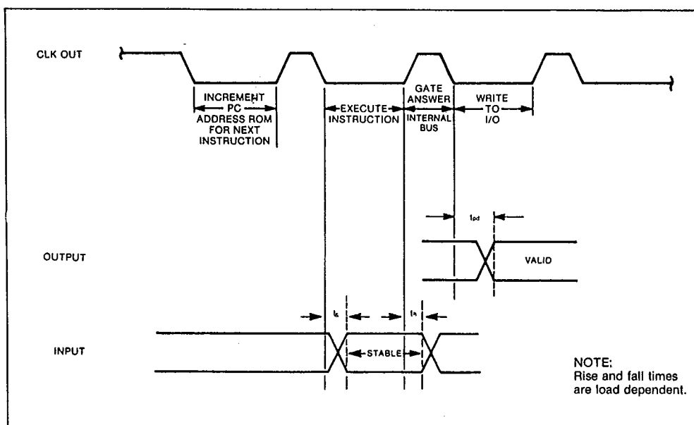
Fig.6 I/O timing
