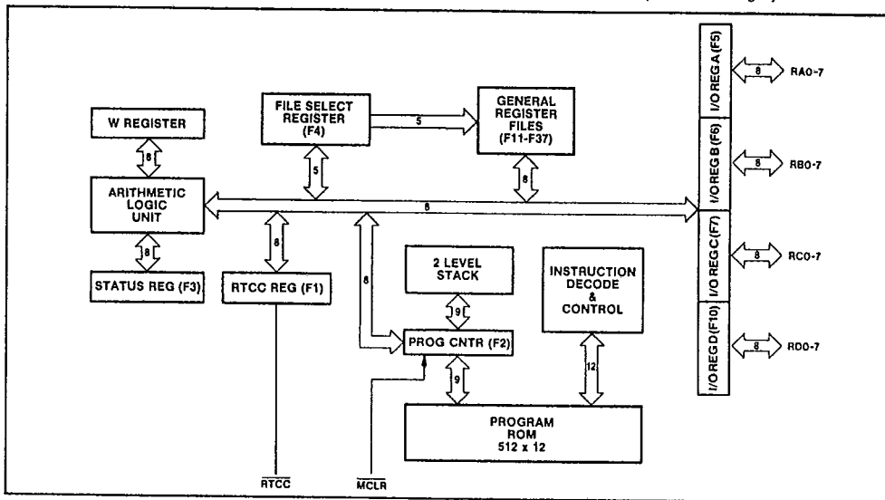
Fig. 2 PIC1650A block diagram
