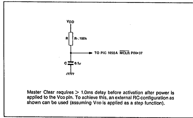
Fig.13 Master clear
