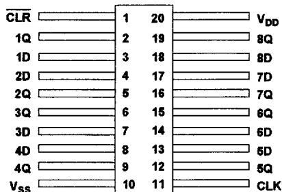
20-Lead Flatpack Top View
