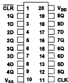
20-Lead Flatpack Top View
