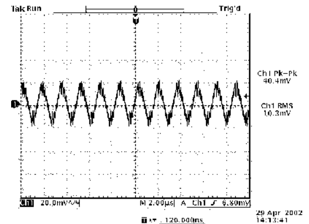
Ripple and noise at full load and 3.3Vdc input, 1.2Vdc output and T_a=25^\circ\text{C}
