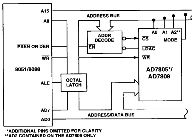
Figure 40. AD7805/AD7809-8051/8088 Interface
