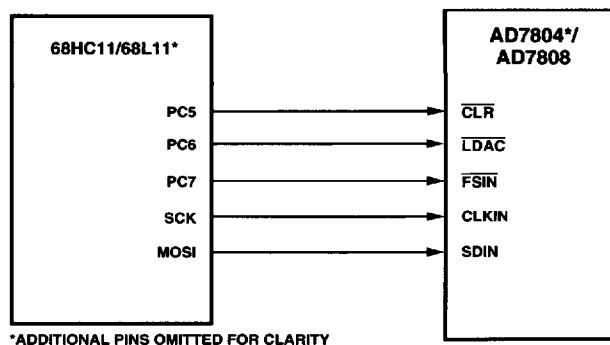
Figure 36. AD7804/AD7808–68HC11/68L11 Interface
