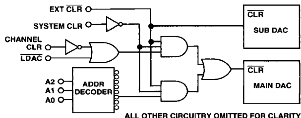
Figure 20. CLR Functions for MAIN and SUB DACs
