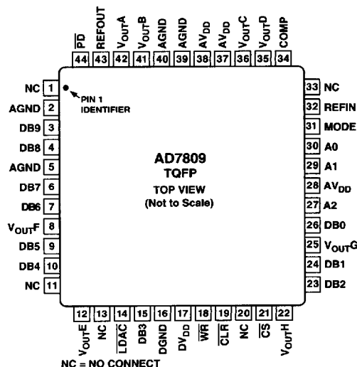
AD7809 PIN CONFIGURATION
