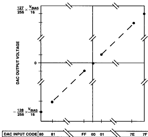
Figure 23. Sub DAC Output Voltage vs. DAC Input Codes (HEX) for Twos Complement Coding
