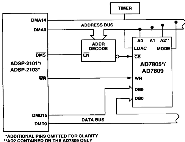
Figure 38. AD7805/AD7809-ADSP-2101/ADSP-2103 Interface
