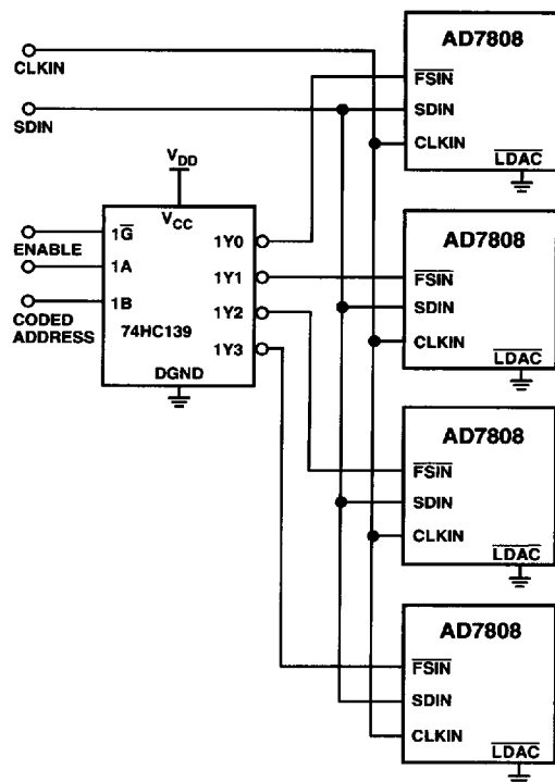
Figure 42. Decoding Multiple AD7808s Using the \overline{\text{FSIN}} Pin
