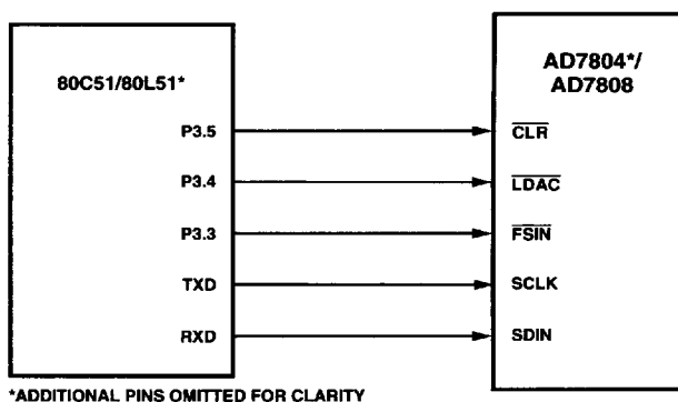
Figure 37. AD7804/AD7808–80C51/80L51 Interface
