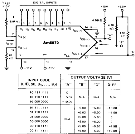
Figure 5. Resistive Output Connections. LIC-250
