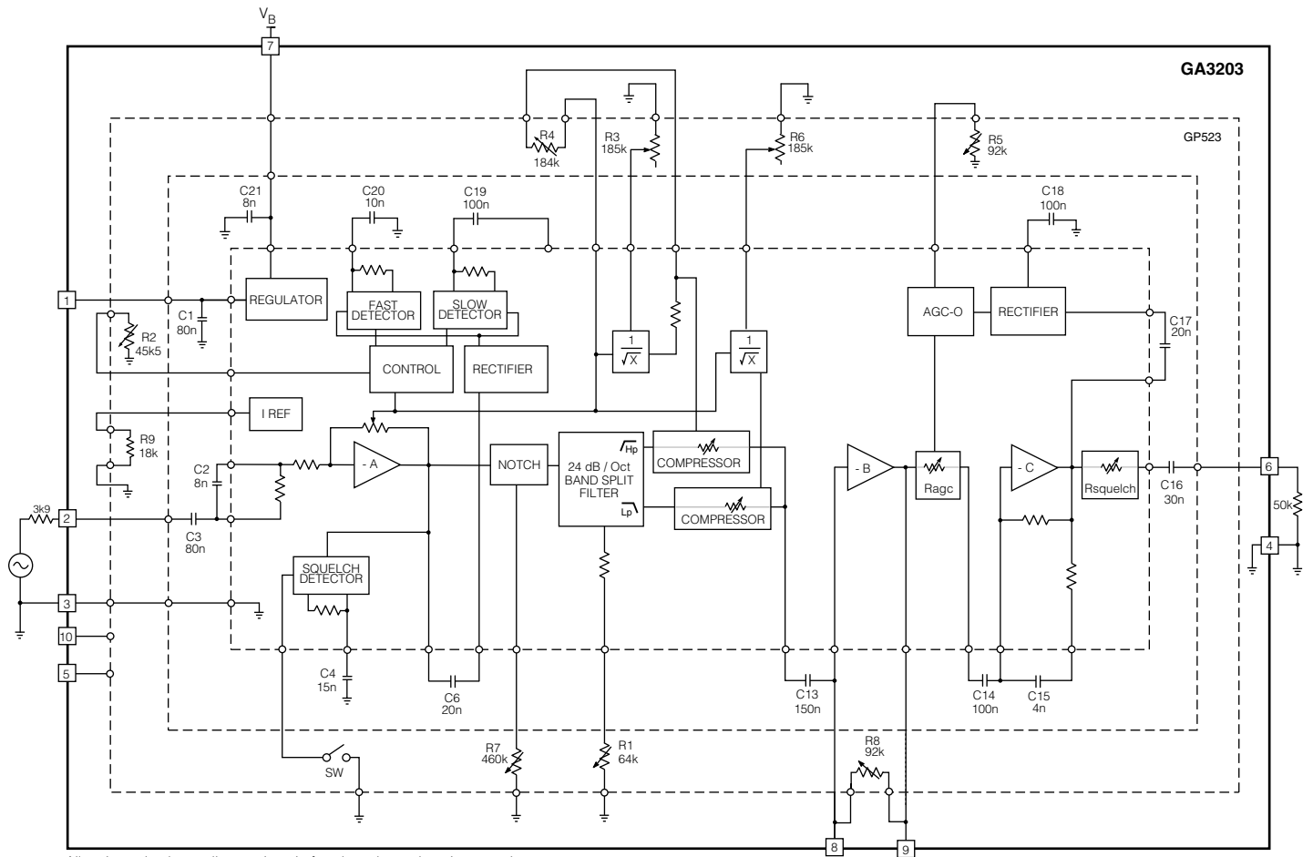
Fig. 1 Test Circuit
