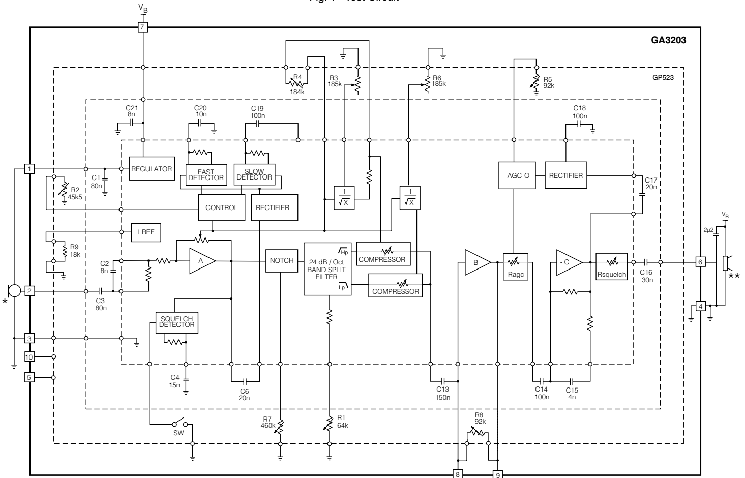
Fig. 1 Test Circuit
