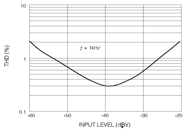
Fig. 9 THD & Noise vs Input Level
