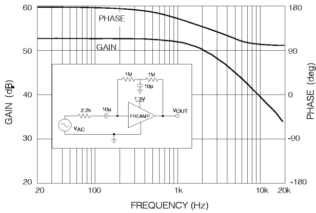
Fig. 11 Stage A Open Loop Gain & Phase vs Frequency
