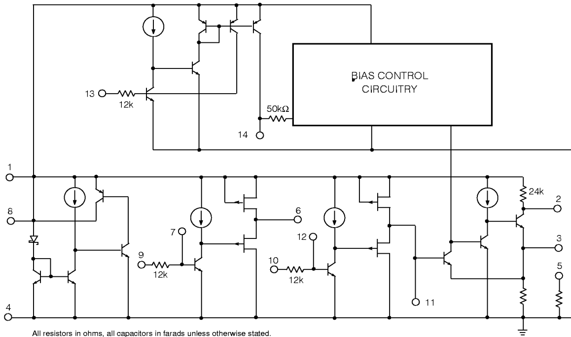
Fig. 2 Functional Schematic Diagram
