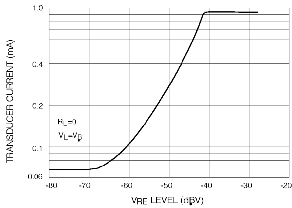
Fig. 7 Transducer Current Characteristics
