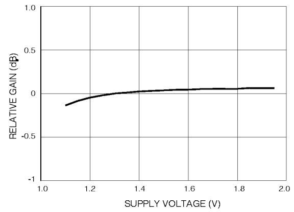
Fig. 8 System Gain vs Supply
