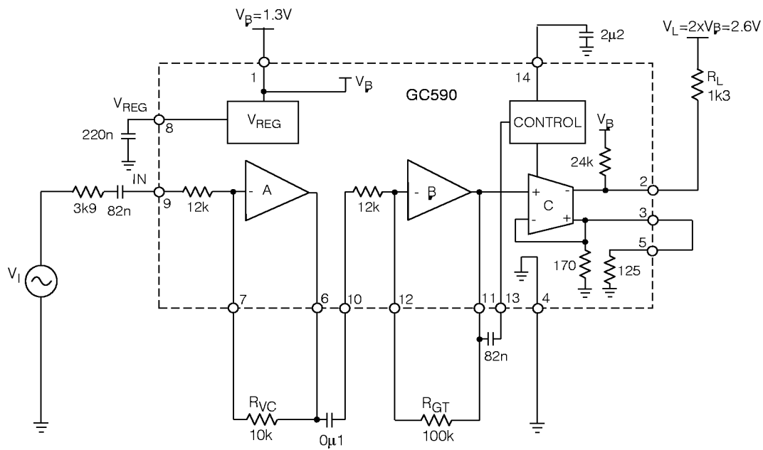
Fig. 4 Characterization Circuit
