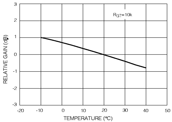
Fig. 14 Relative Gain vs Temperature
