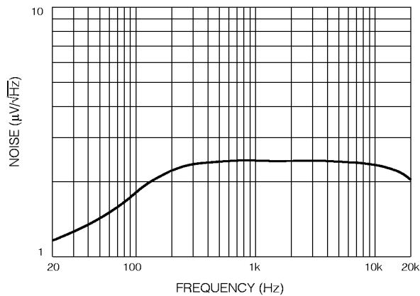
Fig. 13 Output Noise vs Frequency
