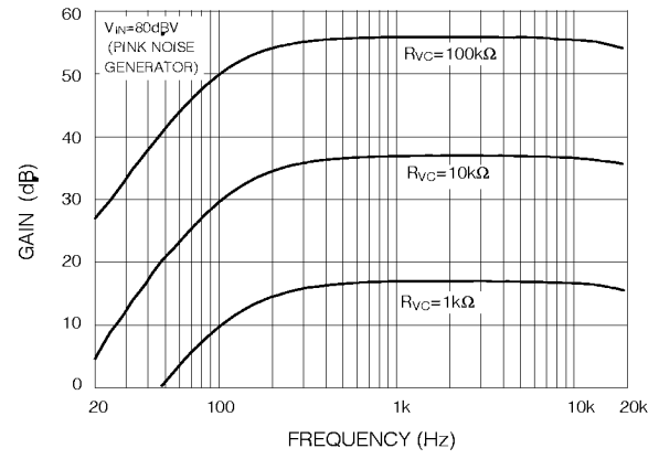
Fig. 6 Frequency Response for Different R_{VC} Values
