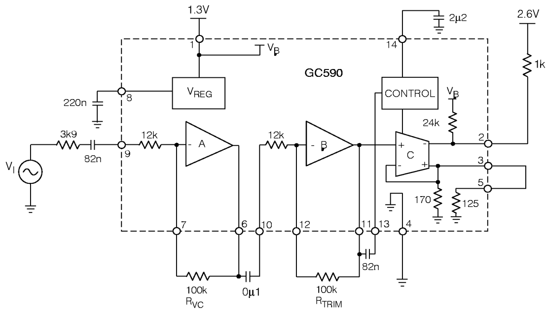
Fig. 1 Test Circuit
