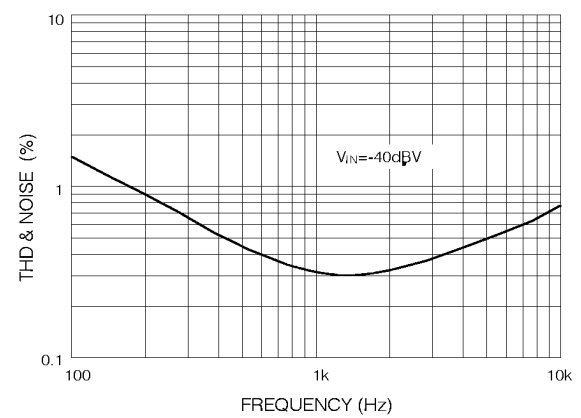
Fig. 10 THD & Noise vs Frequency
