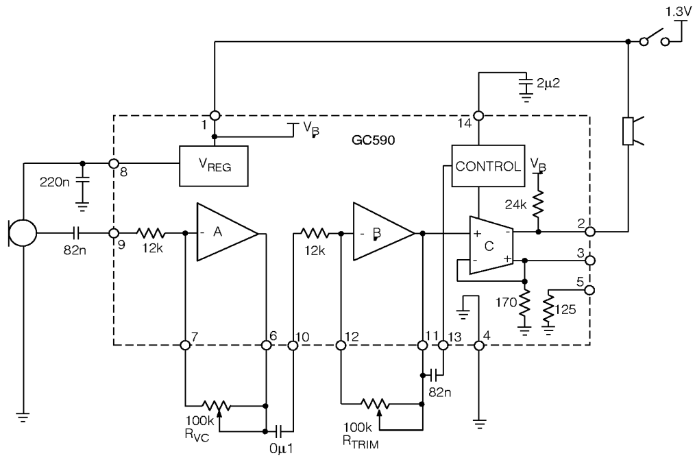
Fig. 3 Typical Hearing Instrument Application
