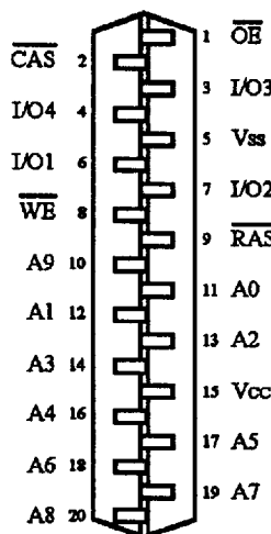
20 ZIP
