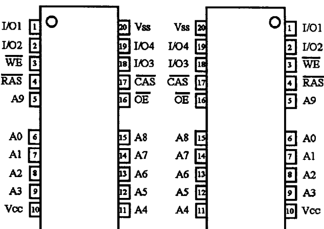
GM71C4400BT/BLT
