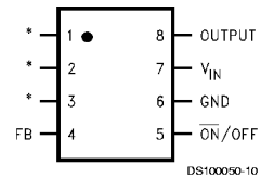
8-Lead Surface Mount (M)
