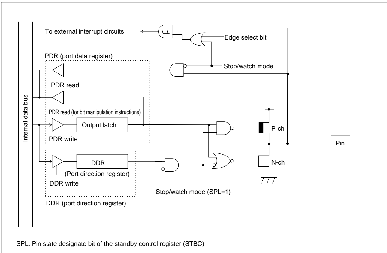
Figure 4.10-2 Block Diagram of Pins of Port 8 (P80 to P83)
