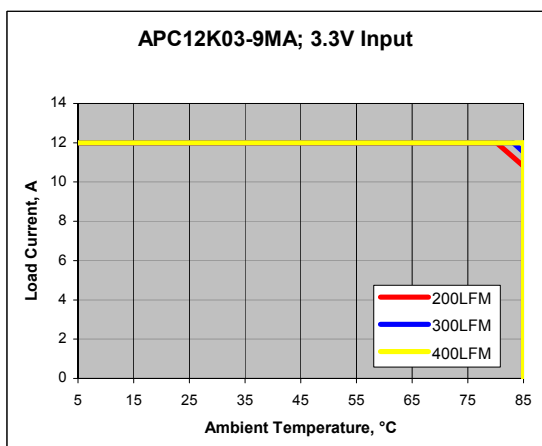
Figure 23. K03 - Load current vs. ambient temp.
