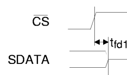
Output Float Delay SSC Mode (Note 19)
