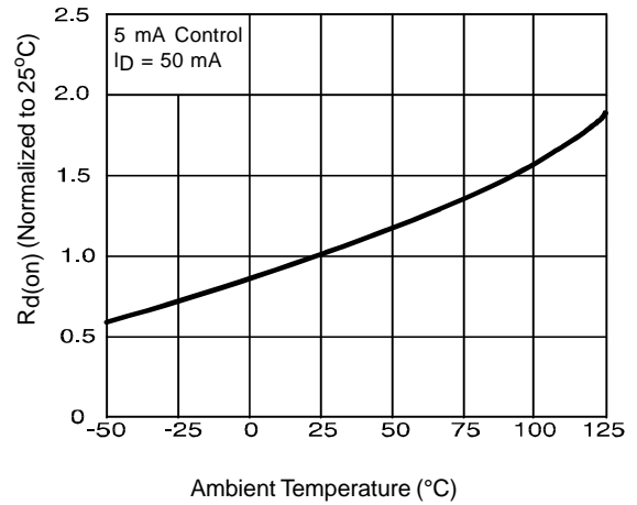
Figure 2. Typical On-Resistance
