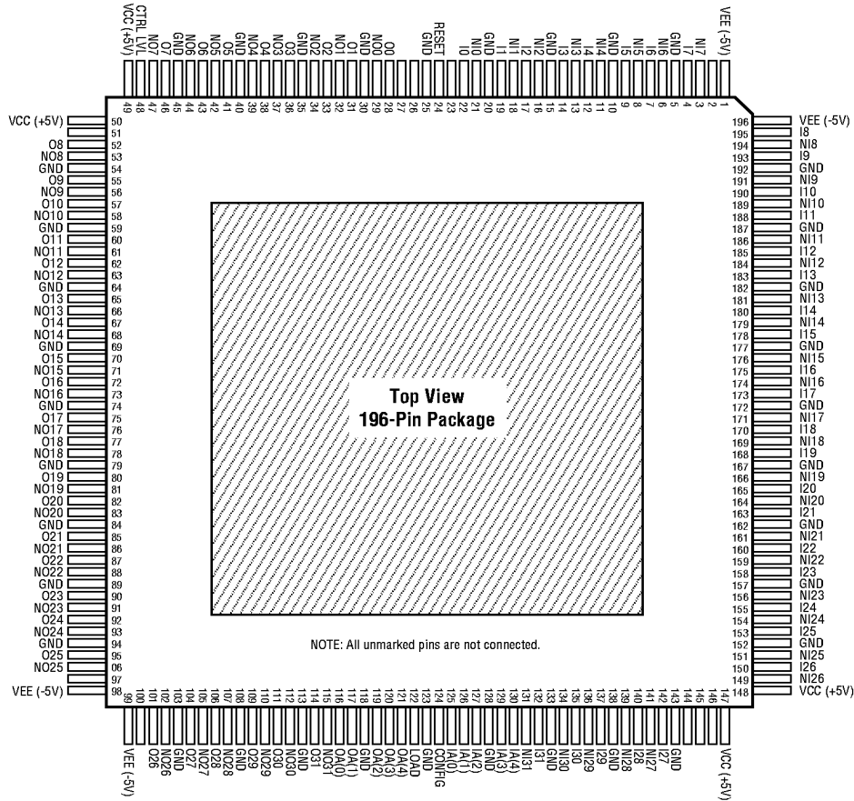
Figure 2. Package Pinout
