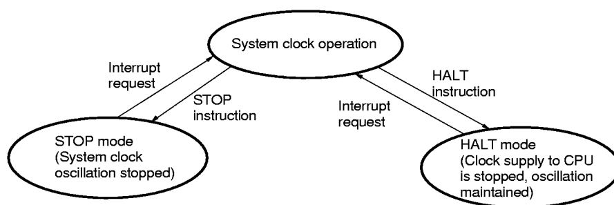
Figure 8-1. Standby Function
