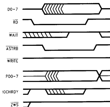
FIGURE 7-2. EPP 1.7 Address Read
