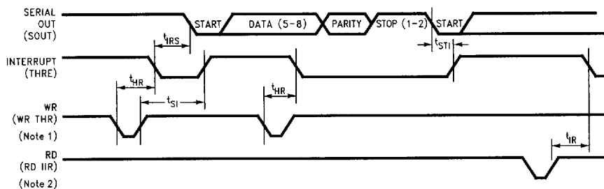
FIGURE 9-5. Transmitter Timing
