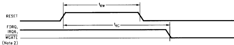
FIGURE 9-9. Reset Timing
