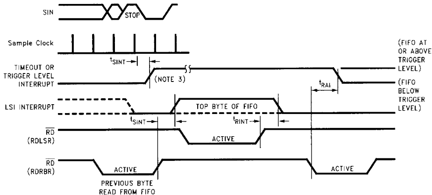
FIGURE 9-6d. Timeout Receiver Timing
