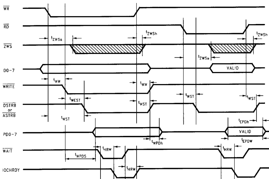
FIGURE 9-17. Enhanced Parallel Port Timing
