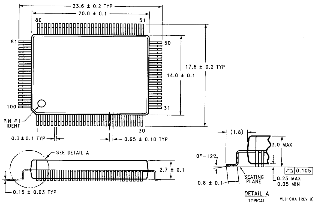
Plastic Quad Flatpak (EIAJ) (PQFP) Order Number PC87332VLJ or PC87332VLJ-5 NS Package Number VLJ100A
