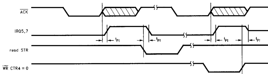
FIGURE 9-15. Extended Mode Parallel Port Interrupt Timing
