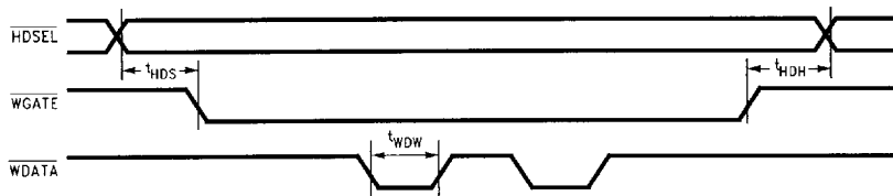
FIGURE 9-10. Write Data Timing
