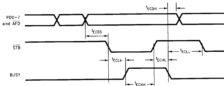
FIGURE 9-18. ECP Parallel Port Forward Timing Diagram
