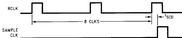
FIGURE 9-6a. Sample Clock Timing
