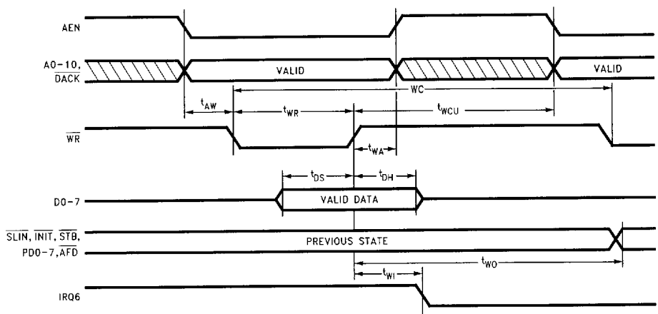
FIGURE 9-3. Microprocessor Write Timing
