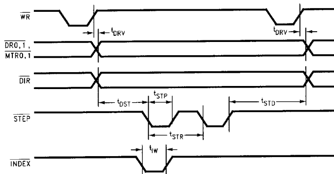
FIGURE 9-11. Drive Control Timing
