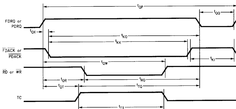
FIGURE 9-8. DMA Timing
