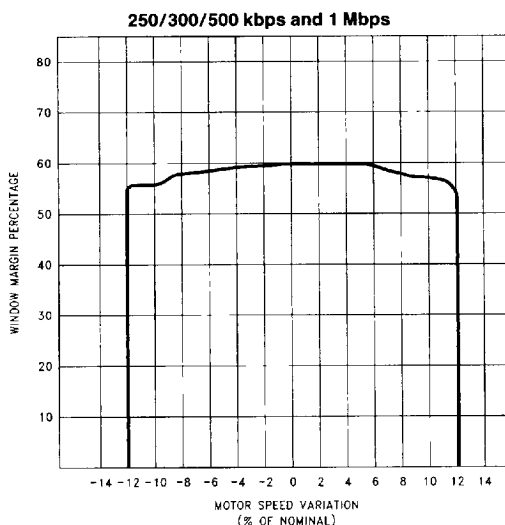
FIGURE 5-1. PC87332 Dynamic Window Margin Performance (Typical Performance at V_{DD} = 5.0V , 25^{\circ}C )
