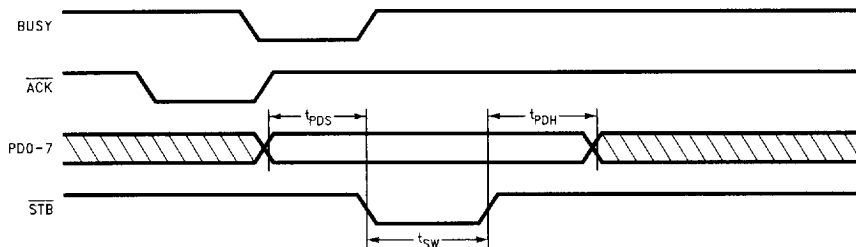
FIGURE 9-16. Typical Parallel Port Data Exchange
