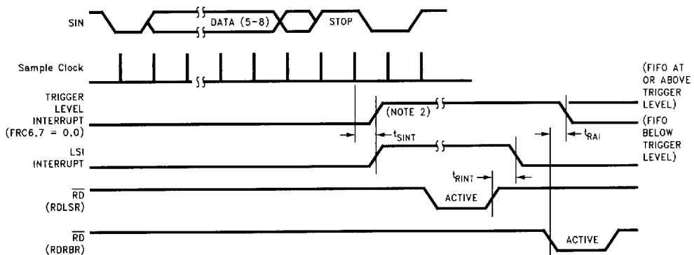
FIGURE 9-6b. Receiver Timing
