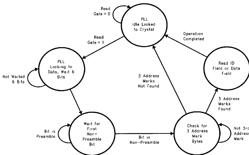
FIGURE 5-2. Read Data Algorithm—State Diagram
