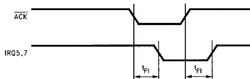
FIGURE 9-14. Compatible Mode Parallel Port Interrupt Timing
