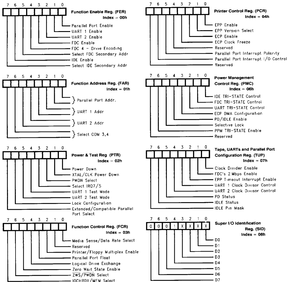
FIGURE 2-1. PC87332VLJ/PC87332VLJ-5 Configuration Registers
