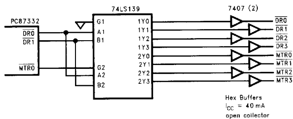
FIGURE 2-2. PC87332 Four Floppy Drive Circuit Example
