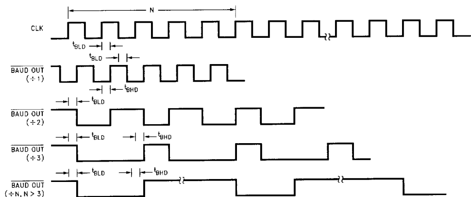
FIGURE 9-4. Baud Out Timing
