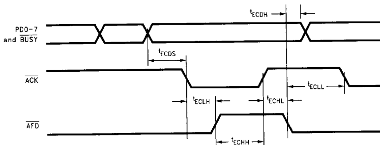
FIGURE 9-19. ECP Parallel Port Backward Timing Diagram
