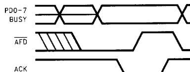
FIGURE 7-7. ECP Backward Read Cycle
