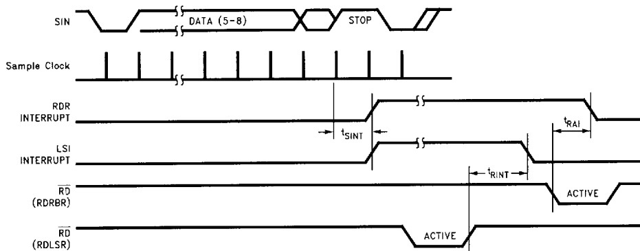
FIGURE 9-6b. Receiver Timing
