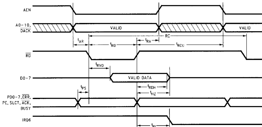
FIGURE 9-2. Microprocessor Read Timing
