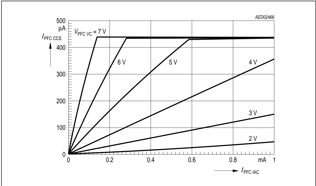
Figure 7 Multiplier Linearity
