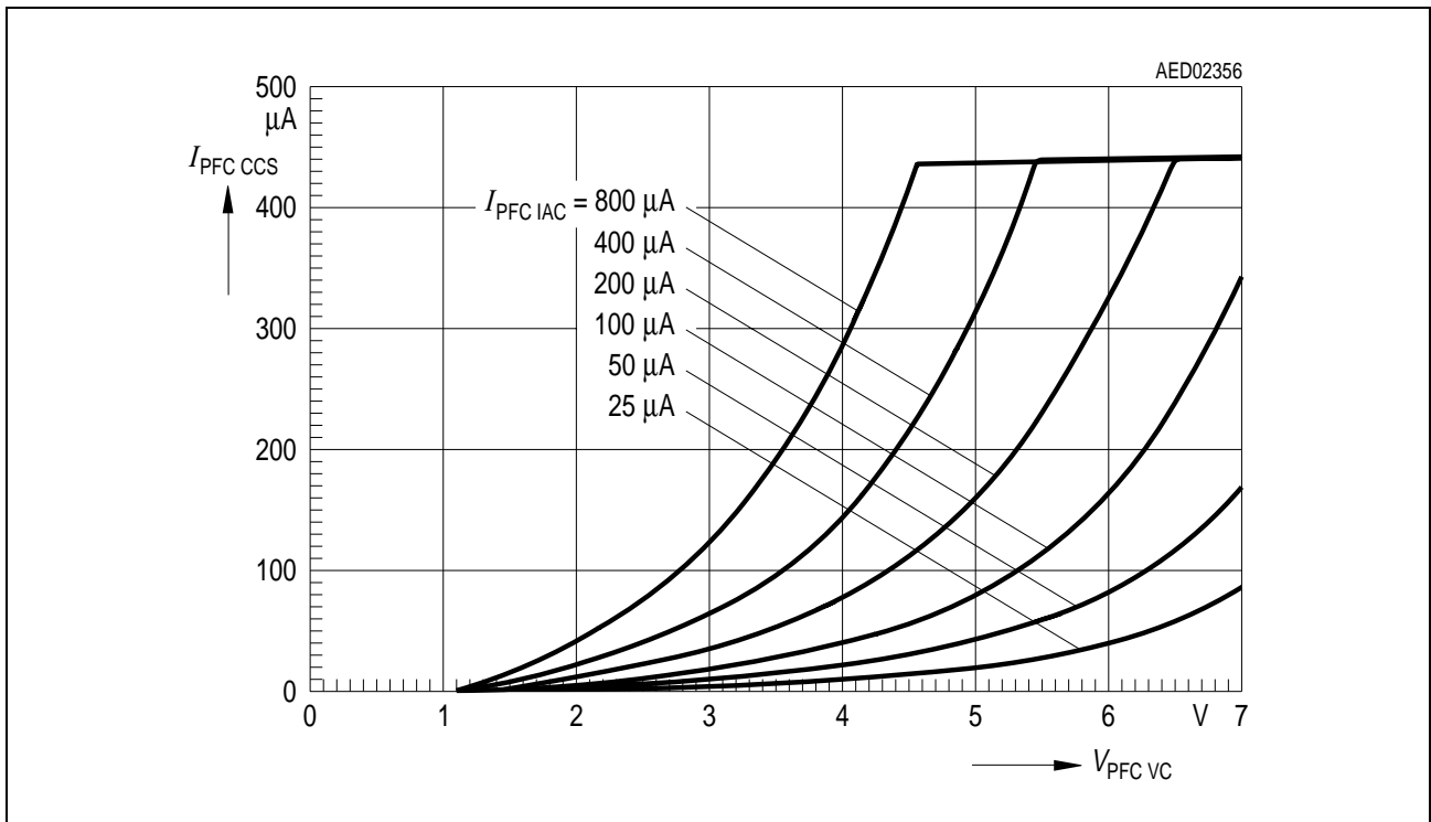
Figure 8 Multiplier Dynamic
