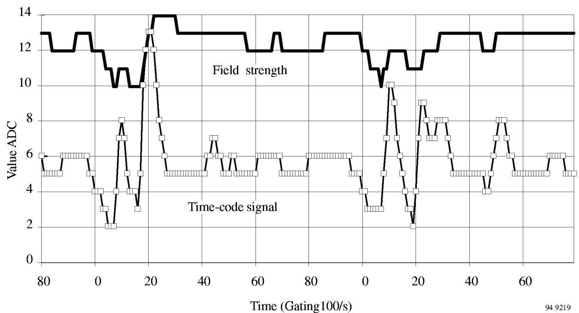
Figure 19. Example of a disturbed DCF signal
