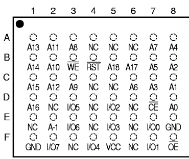
AT49F008A(T) Standard Pin Definition CBGA Top View (Ball Down)
