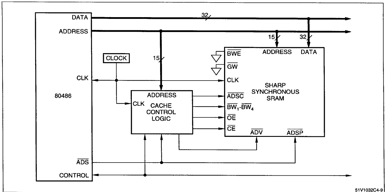
Figure 9. 128K Byte Secondary Burst Mode Cache for 486 Using One LH51V1032 Synchronous SRAM
