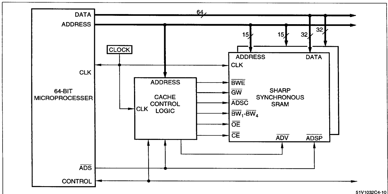
Figure 10. 256K Byte Secondary Burst Mode Cache for Pentium Microprocessor Using Two LH51V1032 Synchronous SRAMs
