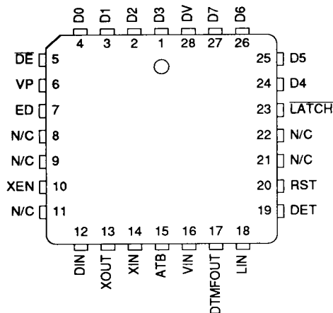
75T2091 28-Pin PLCC
