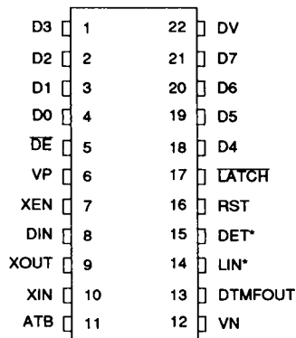
75T2089/2090 22-Pin DIP
