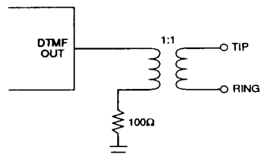
FIGURE 5: DTMF Output
