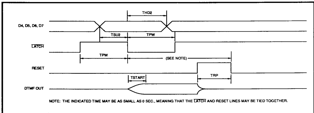
FIGURE 8: DTMF Generator
