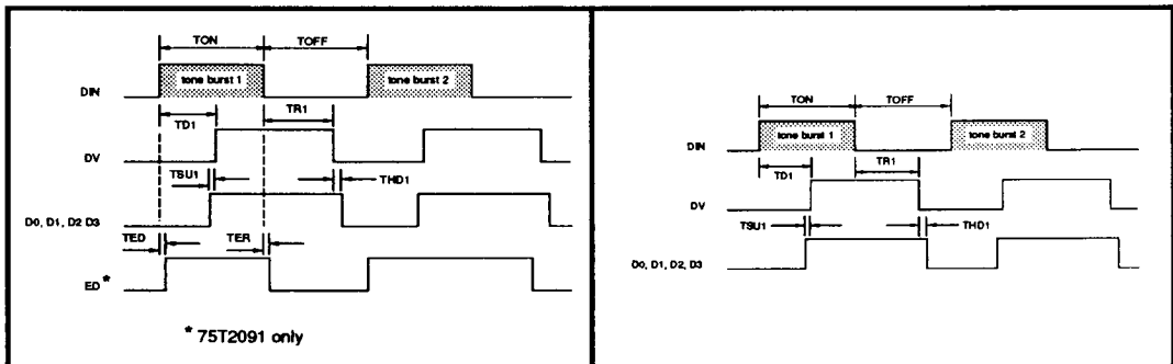
FIGURE 6: DTMF Decoder
