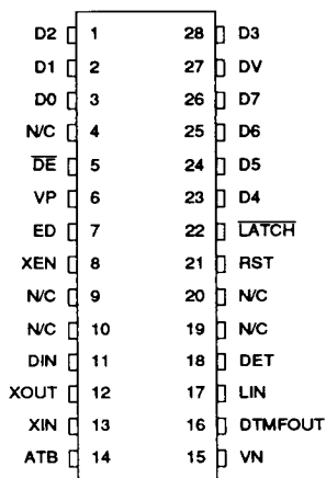
75T2091 28-Pin DIP
