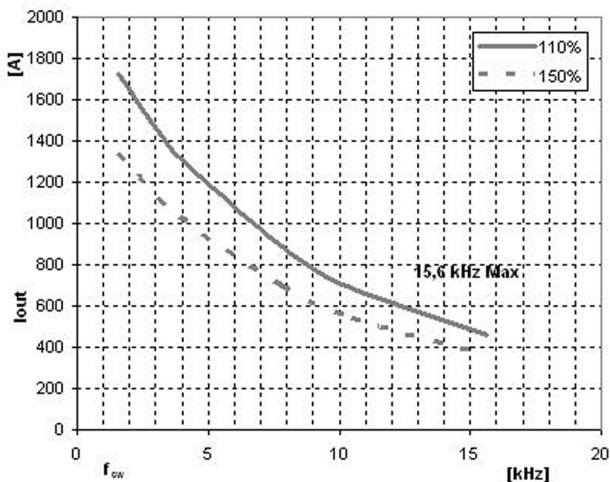
Fig. 3 Max permanent inverter curr. vs. f_{sw} , T_{amb} = 40^\circ C
