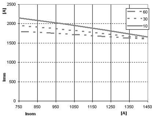
Fig. 1 Maximum overload current, T_{amb} = 40^\circ C
