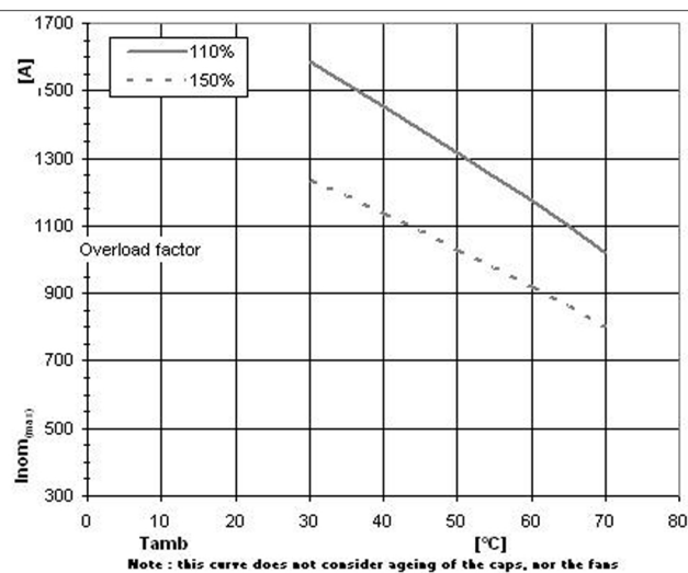
Fig. 5 Max. nominal curr. vs. ambient temperature
