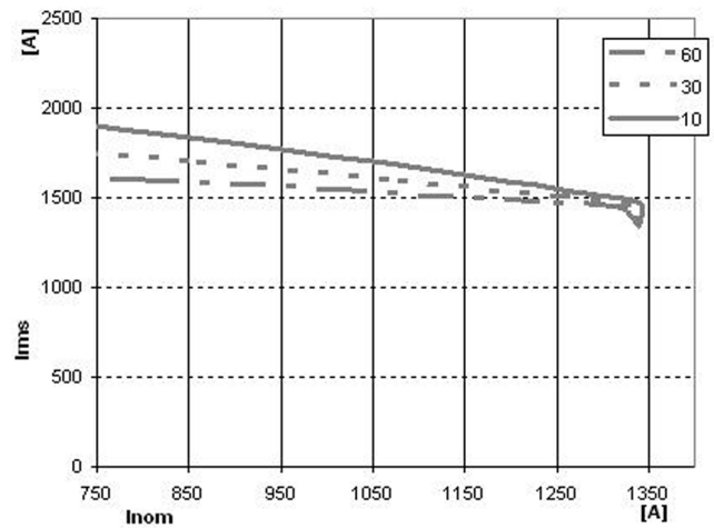
Fig. 2 Maximum overload current, T_{amb} = 50^\circ C
