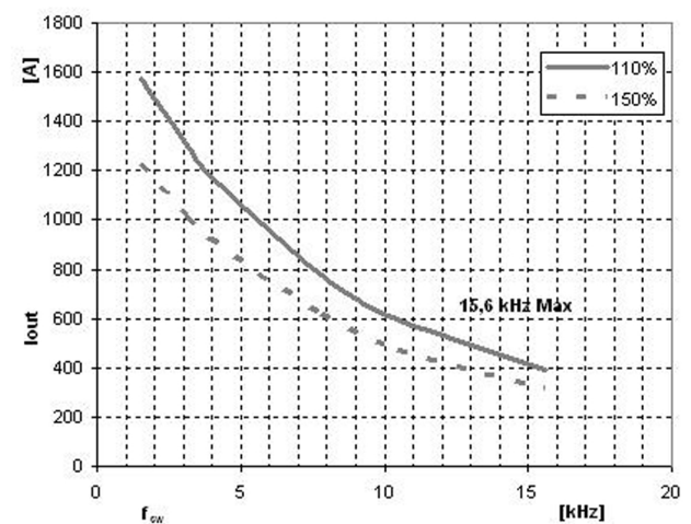
Fig. 4 Max. permanent inverter curr. vs. f_{sw} , T_{amb} = 50^\circ C
