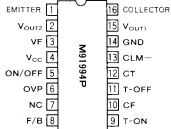
Outline 16P4
