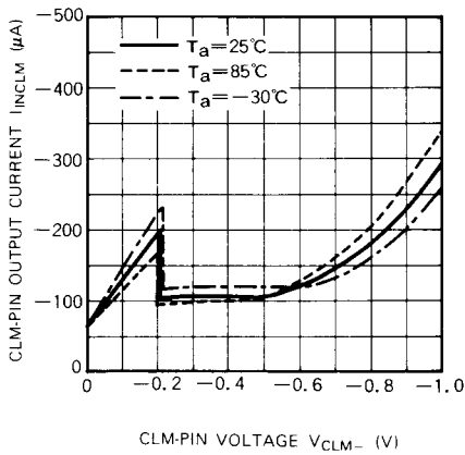
CLM-PIN OUTPUT CURRENT VS. CLM-PIN VOLTAGE
