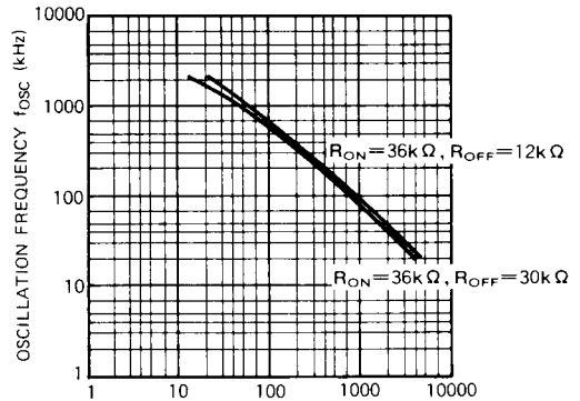
OSCILLATION FREQUENCY VS. CF PIN CAPACITY
