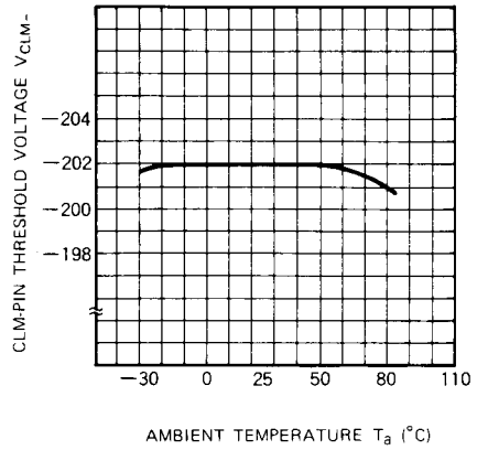
CLM-PIN THRESHOLD VOLTAGE VS. AMBIENT TEMPERATURE
