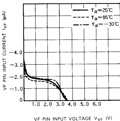
V F PIN INPUT CURRENT VS. INPUT VOLTAGE
