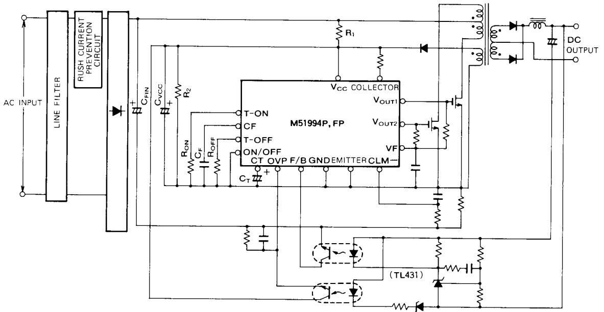
Figure 16 Application circuit for a push-pull regulator
