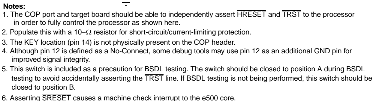
Figure 62. JTAG Interface Connection
