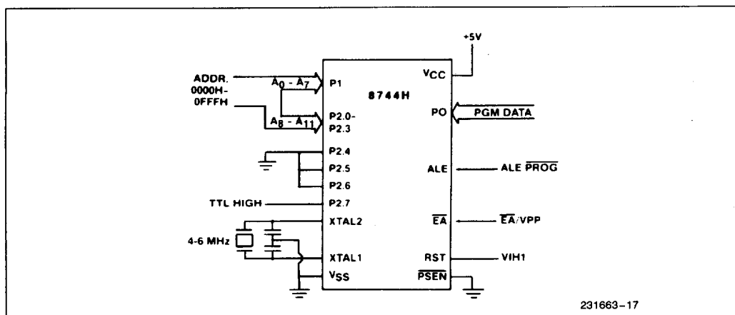
Figure 8. Programming Configuration
